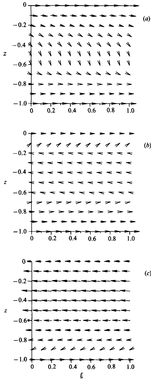
FIGURE 3. Projection of mass transport velocity on plane (a) \zeta = 0 , (b) \zeta = \frac{1}{2}\pi and (c) \zeta = \pi for \theta = 45^\circ , h = 1.0 , and \delta = 0.1 .
