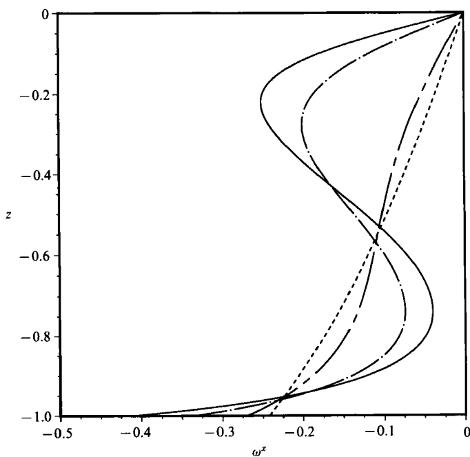
FIGURE 11. Vertical profile of vorticity, \omega^x , at \xi = \zeta = \frac{1}{2}\pi for (a) \delta = 0.04 (—), (b) \delta = 0.05 (— · —), (c) \delta = 0.10 (---), and (d) \delta = 100.0 (- · - · -). \theta = 45^\circ , h = 1.0 .
