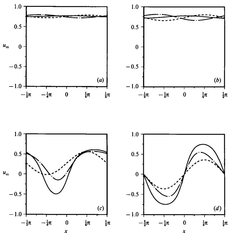
FIGURE 5. Mass transport velocity at free surface y = 0 for \delta equal to 0.04 (—), 0.1 (— · —) and 100 (---); (a) R = 0.1 , (b) R = 0.2 , (c) R = 0.8 , (d) R = 1.0 .
