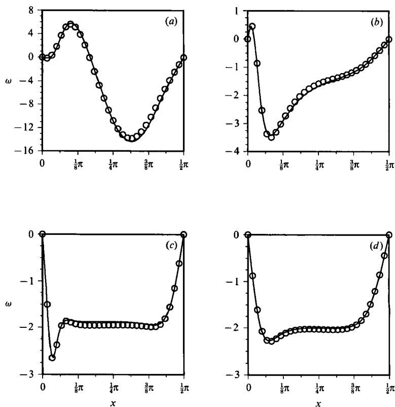
FIGURE 2. Horizontal profile of the vorticity under a standing wave for \delta = 0.04 , from the spectral scheme (—), and FEM scheme ( \bigcirc ) at (a) y = -1.0 (seabed), (b) y = -0.9 , (c) y = -0.6 , (d) y = -0.2 .
