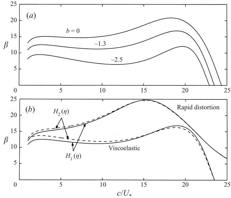
FIGURE 3. (a) Using the viscoelastic limit ( I = 0 ) from figure 2(a), the parameter b is varied as a test of sensitivity. Note that b = -1.3 is a generally accepted value. (b) Two parameterizations of the wave-following coordinate: the solid lines (curves taken from figure 2b) use the simple exponential form H_1(\eta) , the dashed lines show the slight changes with the more elaborately constructed H_2(\eta) .
