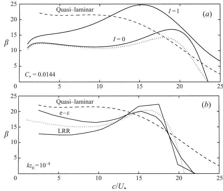
FIGURE 2. (a) The solution of (5.2)–(5.4) for the logarithmic velocity profile with Charnock's C_* = 0.0144 and three different choices of I : I = 1 , the rapid-distortion approximation carried all the way to the surface; I = 0 , the present viscoelastic limit; and I = 1 - \exp(-\eta) , an interpolation between these limits. The quasi-laminar result (---) is shown for comparison. (b) Two closure models after Mastenbroek (1996): the e-\epsilon model and the Launder et al. model. The dotted line is the prediction derived from Townsend's (1972) model, adjusted to kz_0 fixed at 10^{-4} , the value used in Mastenbroek.
