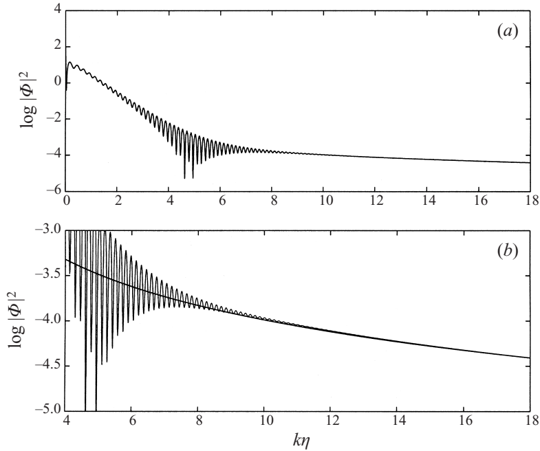
FIGURE 4. Match to two decaying fields at \eta = 18 for c = 15 : (a) shows initial exponential decay followed by algebraic tail; (b) shows closeup of the algebraic tail, with a superposed line that is computed according to the asymptotic expansion in (A 1).
