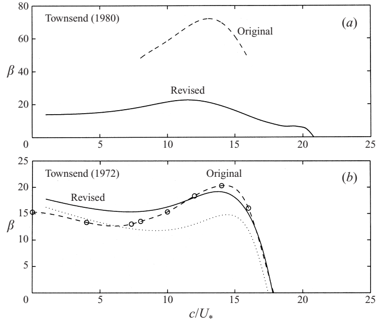
FIGURE 1. A plot of the normalized drag determined from (5.6a) as the sum of the imaginary component of the perturbation pressure and the real component of the perturbation shear stress. (a) Townsend's (1980) rapid-distortion model: the dashed line is the sum of curves in Townsend (1980) figures 6(a) and 6(b) corresponding to KU(k^{-1})/\tau_0^{1/2} = 8 in his notation, and the solid line indicates our revision. (b) Townsend's (1972) viscoelastic model: the circles are directly from Townsend's table 2 on summing the entries labelled P_i and \tau_r , the dashed line is our smoothed fit, the solid line is our revision, and the dotted line is the present viscoelastic approximation ( I = 0 ).
