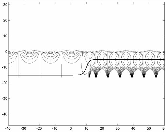
Figure 2 Calculated wave field in the case of oblique waves propagating with direction -30^\circ over a smooth and steep shoal and under the effects of an opposing shear current.
