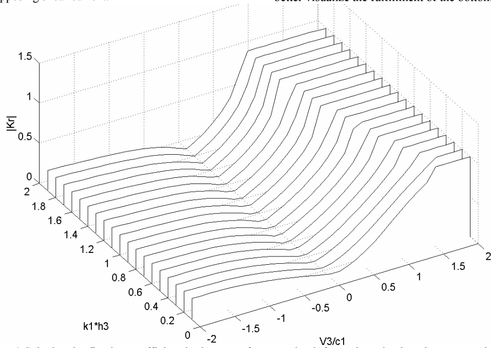
Figure 4 Calculated reflection coefficient in the case of a steep shoal, for various depth and current variations. Incident wave conditions: \kappa_1 h_1 = 4 and \theta_1 = -30^\circ
