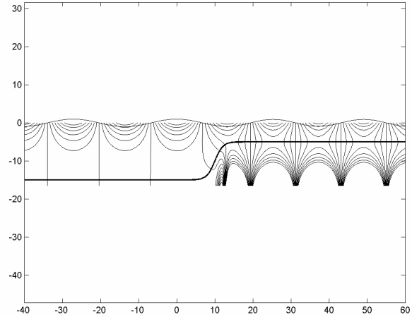
Figure 3 Same as in Fig.2, but without current. The extension of the equipotential lines below the bottom surface is maintained in order to better visualize the fulfillment of the bottom boundary condition.
