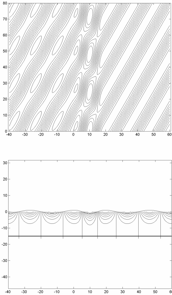
Figure 5 Calculated wave field in the case of oblique waves propagating with direction -30deg in constant depth under the effects of an opposing sinusoidal shear current.
