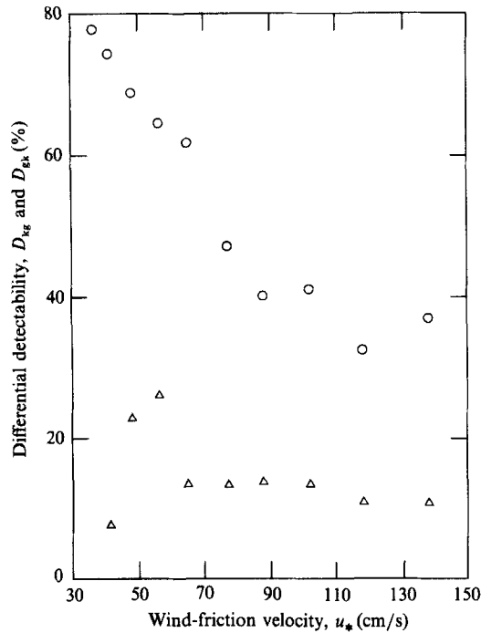
FIGURE 5. Differential detectabilities at various wind-friction velocities. \circ , D_{gk} ; and \triangle , D_{kg} .
