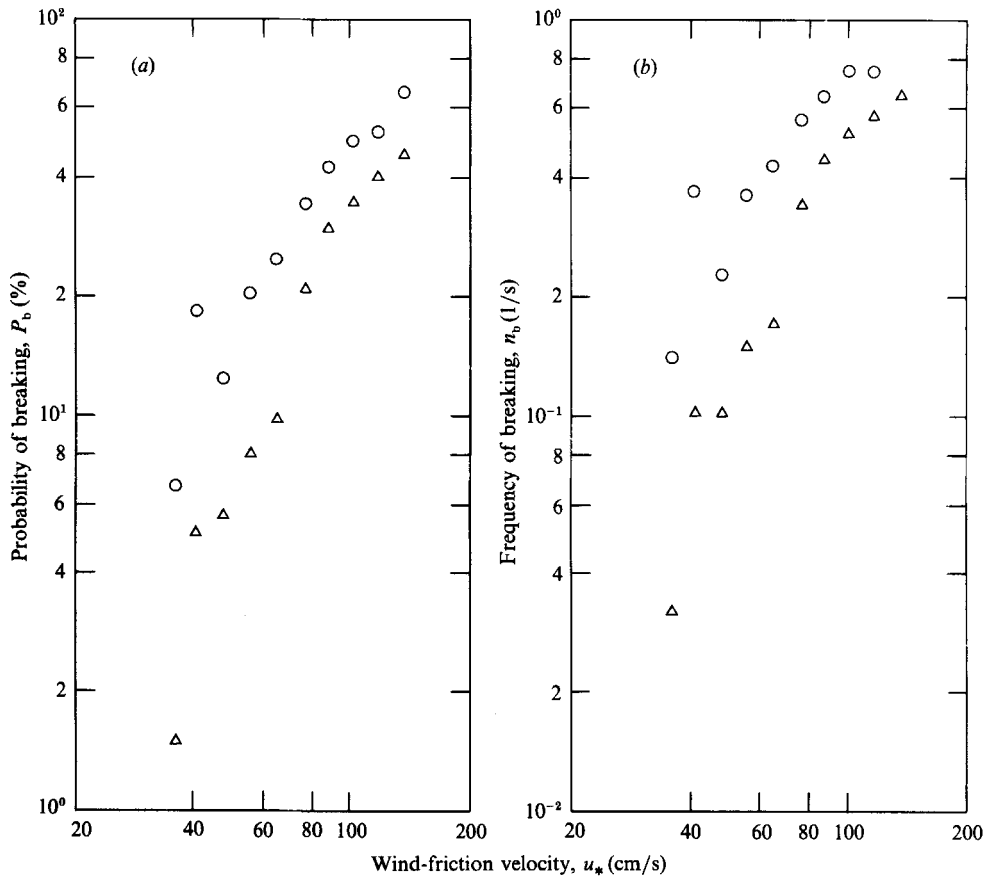
FIGURE 4. (a) Probability and (b) frequency of breaking occurrence at various wind-friction velocities. The data analysed with the geometric criterion are indicated by ○, and the kinematic criterion by △.
