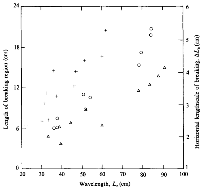
FIGURE 15. Variation of horizontal lengthscale with wavelength. The data are from the present experiment determined with geometric ( \circ ) and kinematic ( \triangle ) criteria; and from Duncan's (1981) horizontal dimension of the breaking region ( + ).
