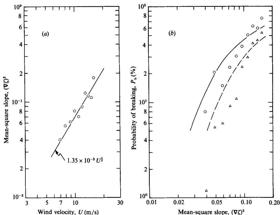
FIGURE 11. Mean square slope and breaking probability. The results are determined with the geometric ( \circ ), and kinematic ( \triangle ) criteria; the solid curve represents the results of Ochi & Tsai (1983), and the dashed curve is the solution of Srokosz (1986) for \alpha = 0.5 .
