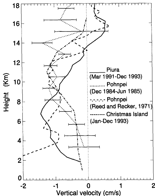
FIG. 10. Mean profiles of the vertical wind from three separate equatorial sites obtained under reasonably clear sky conditions. The Piura profile for the almost 3-yr period discussed in this paper appears as a solid curve. Corresponding profiles for Christmas Island (dashed curve) and Pohnpei (dotted curve) are also plotted. The Christmas Island profile was reproduced from Balsley et al. (1988). Error bars on the Piura and Christmas Island curves are typically smaller than those shown for Pohnpei. The dash-dot curve (Reed and Recker 1971) was obtained for clear sky conditions in the western tropical Pacific using conventional Rawinsonde data and standard convergence techniques. Note that all four curves show comparable 1 \text{ cm s}^{-1} subsidence in the troposphere, suggesting that profilers are capable of this accuracy.
