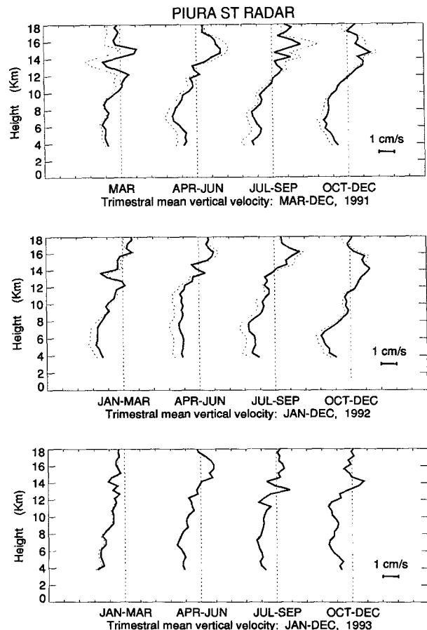
FIG. 4. Plots showing trimestraly averaged mean vertical velocity profiles before (dotted curve) and after (continuous curve) correction for possible contamination by horizontal winds. The dashed vertical lines centered approximately on each set of profiles indicates zero velocity. Values to the right (left) of zero denote upward (downward) velocities. Note that the final three profiles in the lowest panel have not been modified since the antenna was rephased in early February 1993. (January–March 1993 corrections include results both before and after rephasing.)
