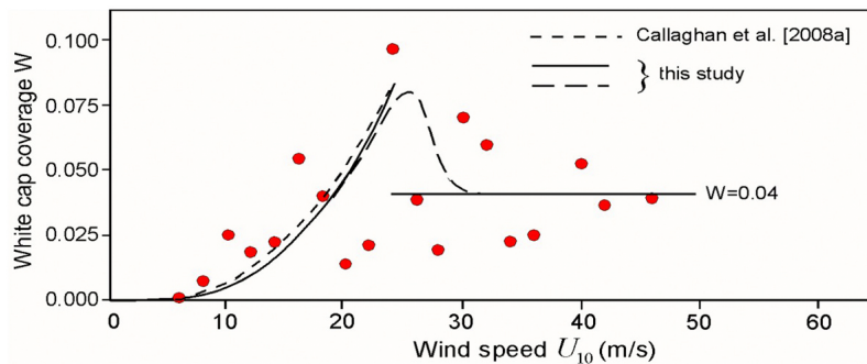
Figure 8. The white cap coverage observations of this study (also in Figure 6C) approximated with a power law for wind speeds U_{10} \leq 24 \text{ m/s} and a constant for U_{10} > 24 \text{ m/s} (solid lines) and a tanh capping with overshoot to a limiting value (long dashes). The two power laws from Callaghan et al. [2008a] concatenated at U_{10} = 10 \text{ m/s} are shown with short dashes.
