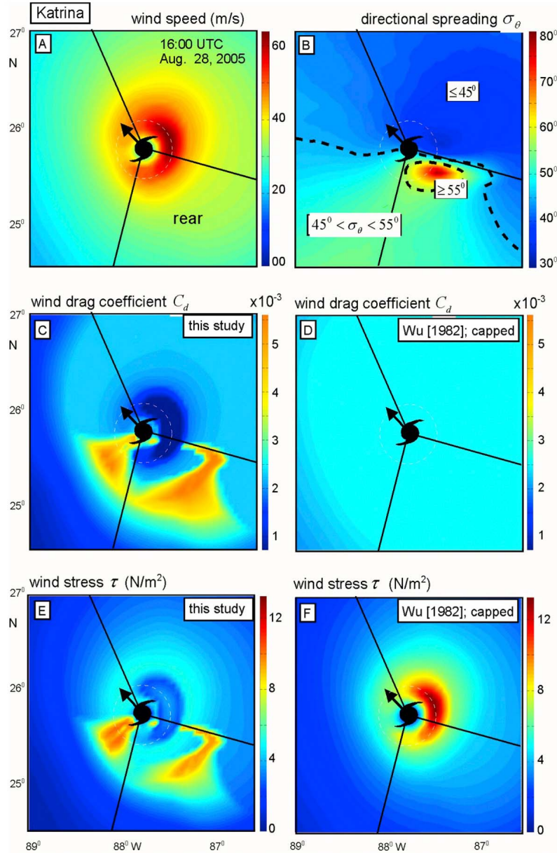
Figure 10. The geographic patterns of wind and waves in hurricane Katrina when it was at its most intense (maximum wind speed U_{10} = 64.2 m/s on Aug. 28, 2005, 16:00 UTC). (a) The wind speed. (b) The wave directional spreading computed with the SWAN wave model. (c and d) The drag coefficient as determined with the expression of equation (1) and (interpolated) coefficients of Table 2 of the present study and with the expression of Wu [1982] (capped at 2.5 \times 10^{-3} ). (e and f) The wind stress determined from the wind speed and the drag coefficients.
