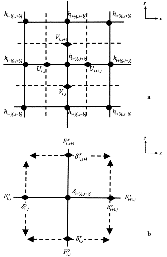
Fig. 2. Grid stencil for discretization of the marine-ice thickness layer evolution equation. (a) The stencil has scalar quantities, i.e. the marine-ice thickness h_{i+\frac{1}{2}, j+\frac{1}{2}} defined by the solid-circle symbols and referred to as the scalar gridpoints, occurring at the intersection of the solid lines. The vector components, i.e. the ice-flow field U_{i,j} and V_{i,j} , defined by the solid-diamond symbols and referred to as the vector gridpoints, occur at the intersection of a solid and a dashed line. This arrangement is known as the C-grid stencil (Arakawa and Lamb, 1977). The grid indices are denoted by subscripts i and j in the \hat{x} and \hat{y} directions, respectively, where full-integer indices occur at the vector gridpoints and half-integers occur at the scalar gridpoints. (b) Stencil definitions for auxiliary variables used in the flux divergence calculation. F_{i,j}^x and F_{i,j}^y are the zonal and meridional volume fluxes and are defined at the vector gridpoints. The grid spacing in the zonal and meridional directions is defined by the “distance” functions \delta_{i,j}^x and \delta_{i,j}^y , respectively, defined at the vector gridpoints. The grid spacing at scalar gridpoints, represented by \delta_{i+\frac{1}{2}, j+\frac{1}{2}} is obtained by averaging neighboring grid spacings as defined at vector points.
