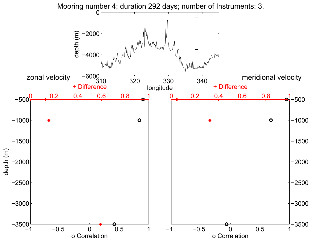
FIG. 16. As in Fig. 14, but for mooring 4 with a record length of 292 days.
