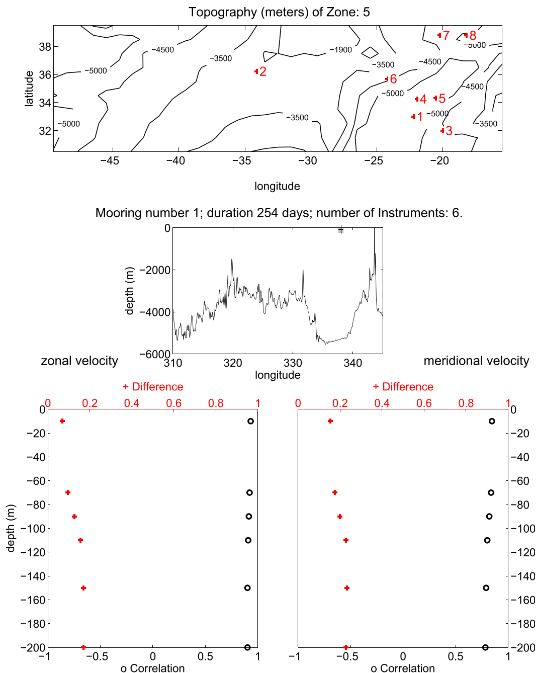
FIG. 12. As in Fig. 10, but for zone 5 with a record length of 254 days.
