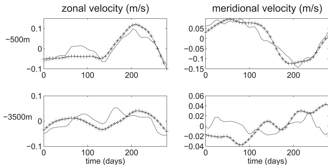
FIG. 17. Zone 5, mooring 4. Time series of the prediction (crosses) and of real data (line) at different depths for (left) zonal and (right) meridional velocity.
