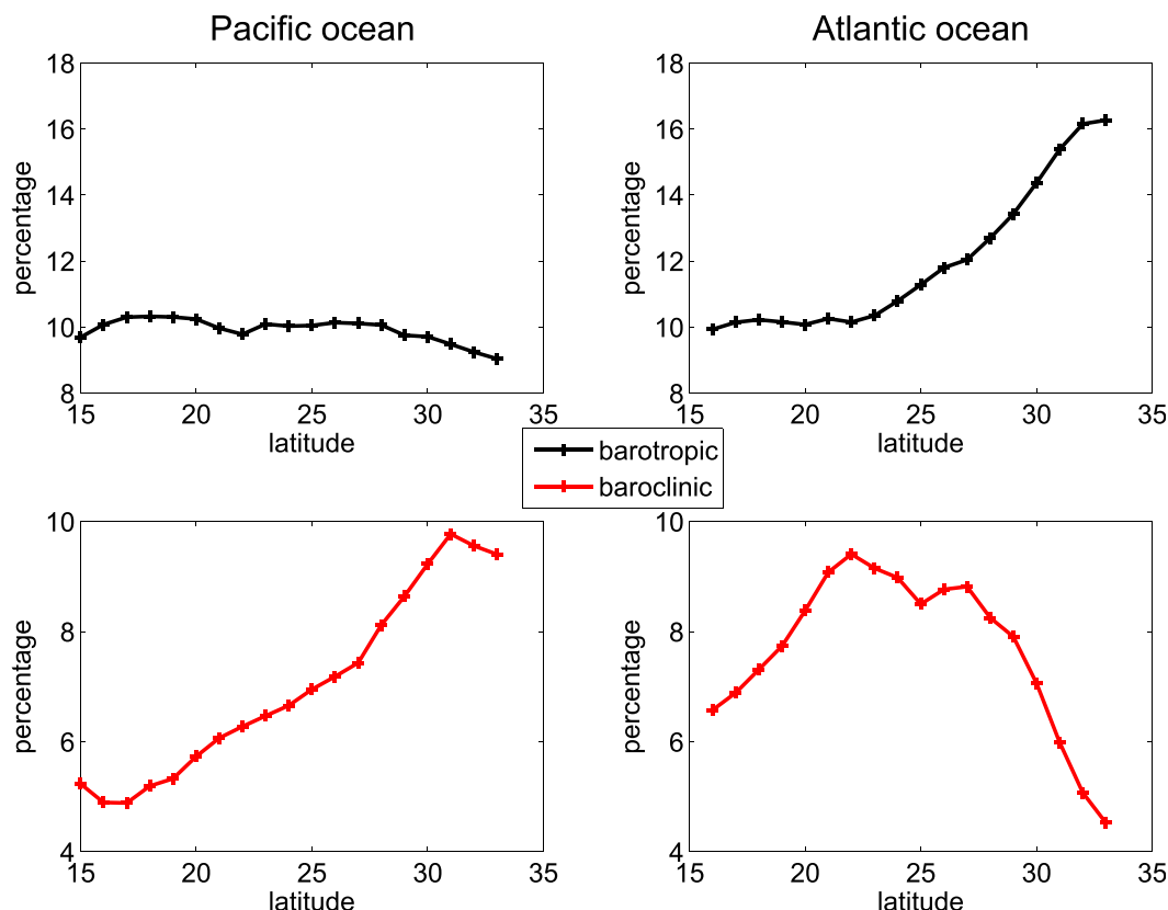
FIG. 20. Percentage of energy that can be attributed to the (top) barotropic and to the (bottom) first baroclinic mode as a function of latitude. (left) Pacific Ocean ( 170^{\circ} to 220^{\circ} ); (right) Atlantic Ocean ( 290^{\circ} to 340^{\circ} ).
