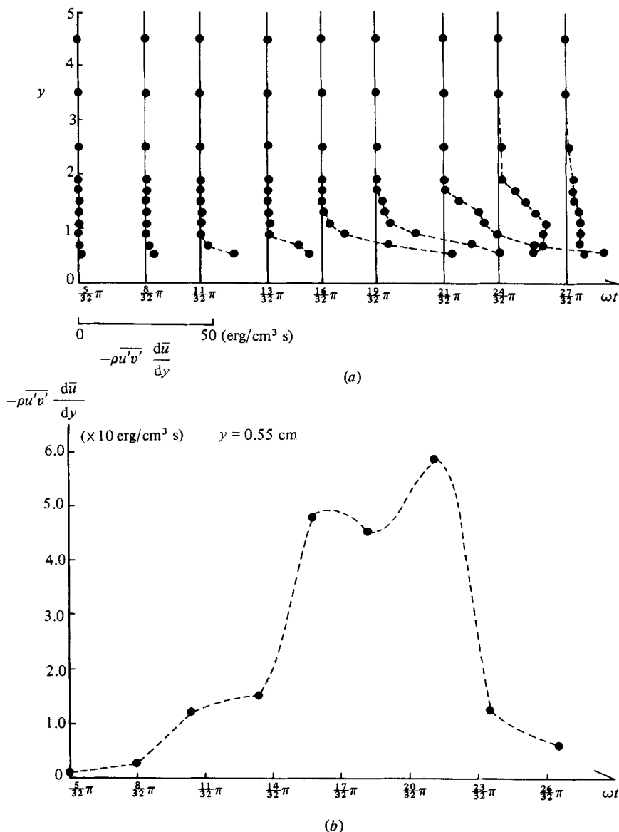
FIGURE 15. (a) Vertical profiles of the turbulence-energy production rate ( -\rho \overline{u'v'} d\bar{u}/dy ). (b) Phase variation of the turbulence-energy production rate at y = 0.55 \text{ cm} .
