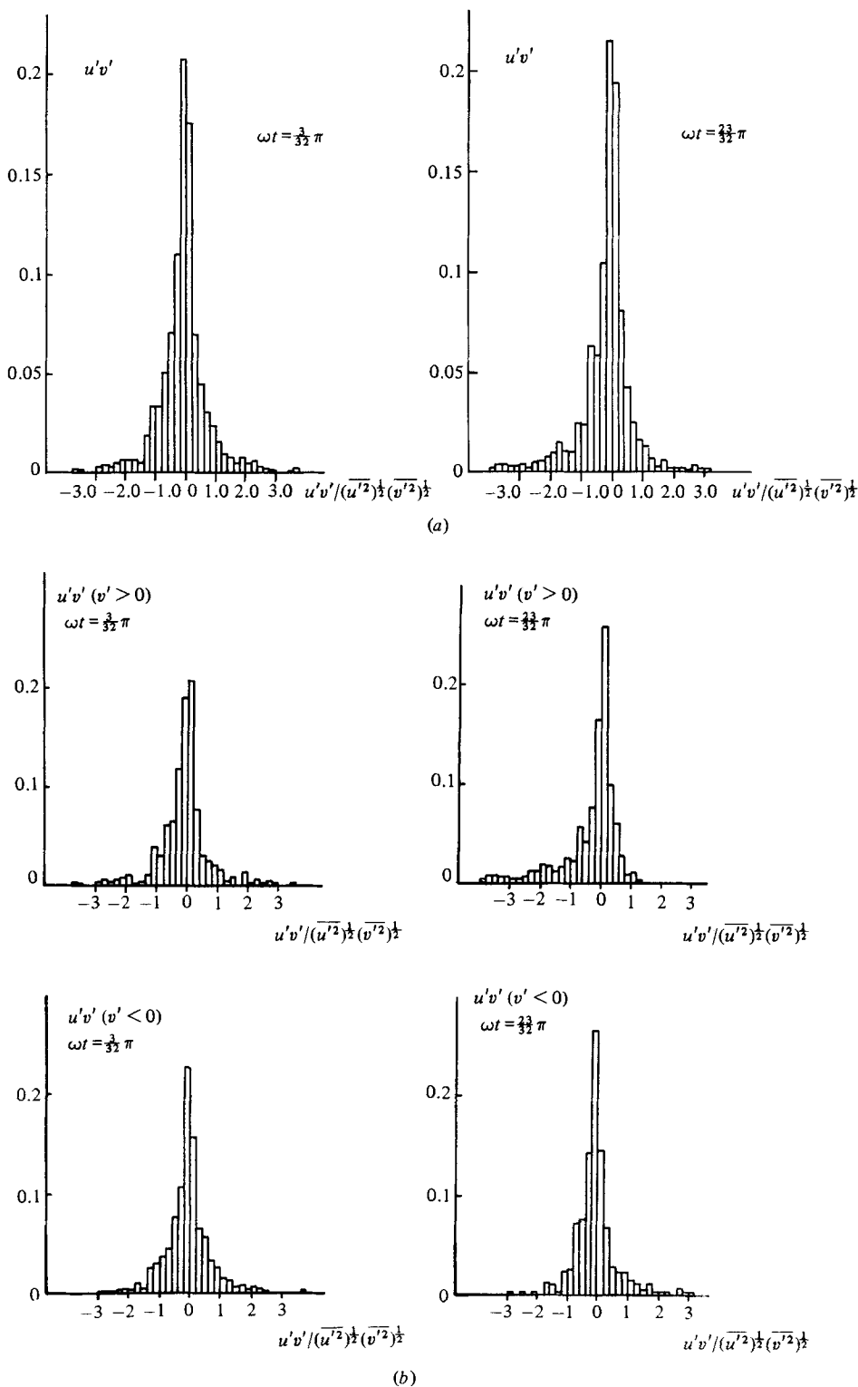
FIGURE 26. Probability density distributions of u'v' at various phases and at y = 0.5 cm: (a) unclassified; (b) classified.
