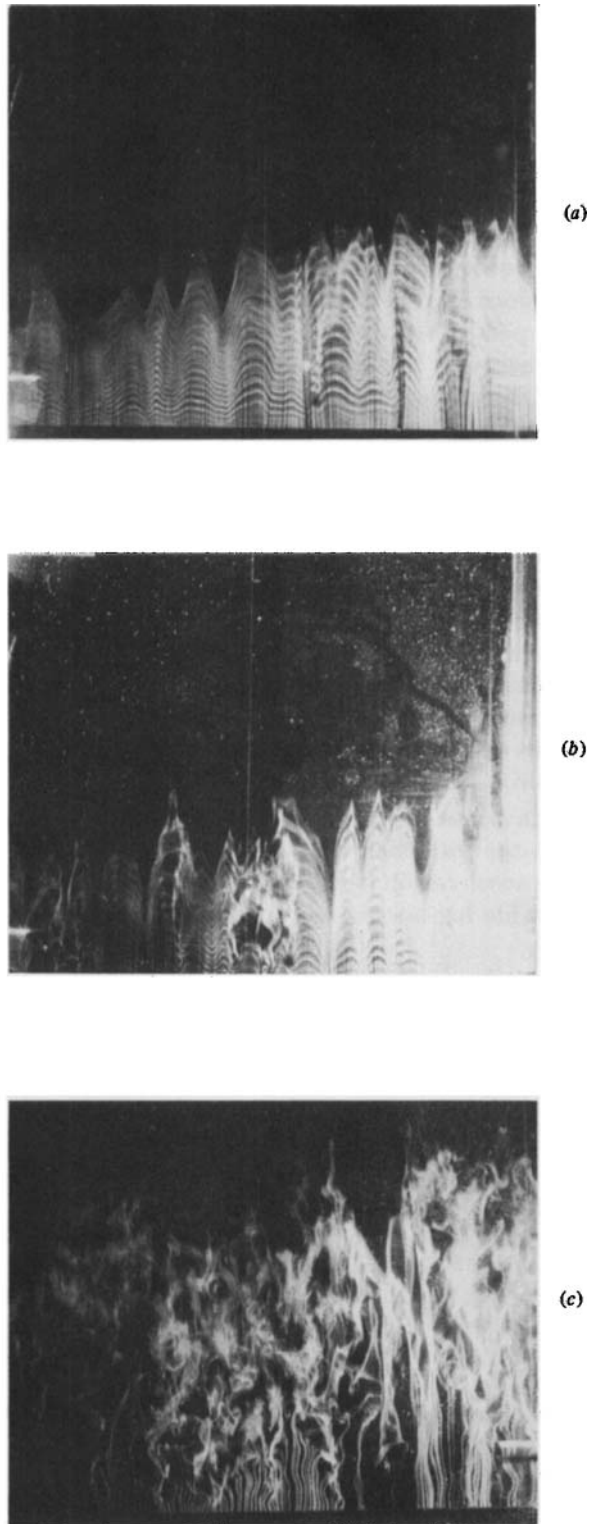
FIGURE 32. Flow visualization in transversal plane of y = 0.3 cm : (a) \omega t = \frac{19}{30}\pi ; (b) \frac{14}{30}\pi ; (c) \frac{13}{30}\pi .
