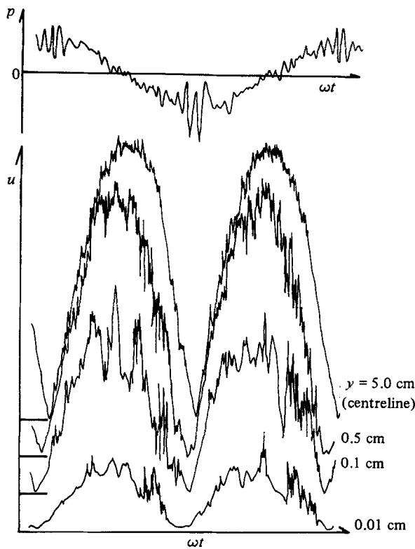
FIGURE 19. Phase variation of the pressure fluctuation compared with the velocity fluctuations.
