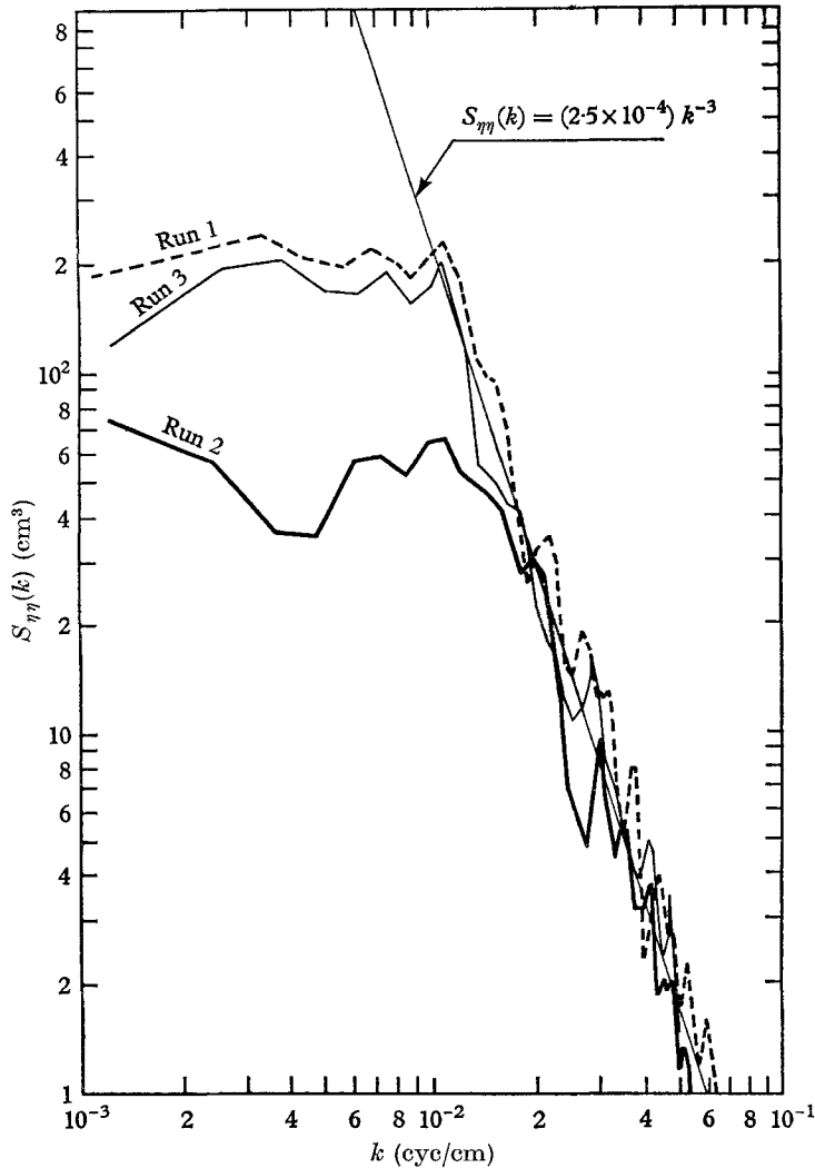
FIGURE 2. Wave-number spectra of sand waves by Ashida & Tanaka (1967) compared with the ‘ -3 power law’ prediction, (10). (The scales of ordinate of the original figures are reduced by a factor ten, because values of variances of elevation \eta^2 obtained by the integration of the spectra are larger just by a factor ten than the values of \sigma^2 = \bar{\eta}^2 listed in table 2 of their original paper which are reasonable values from our experience.)
