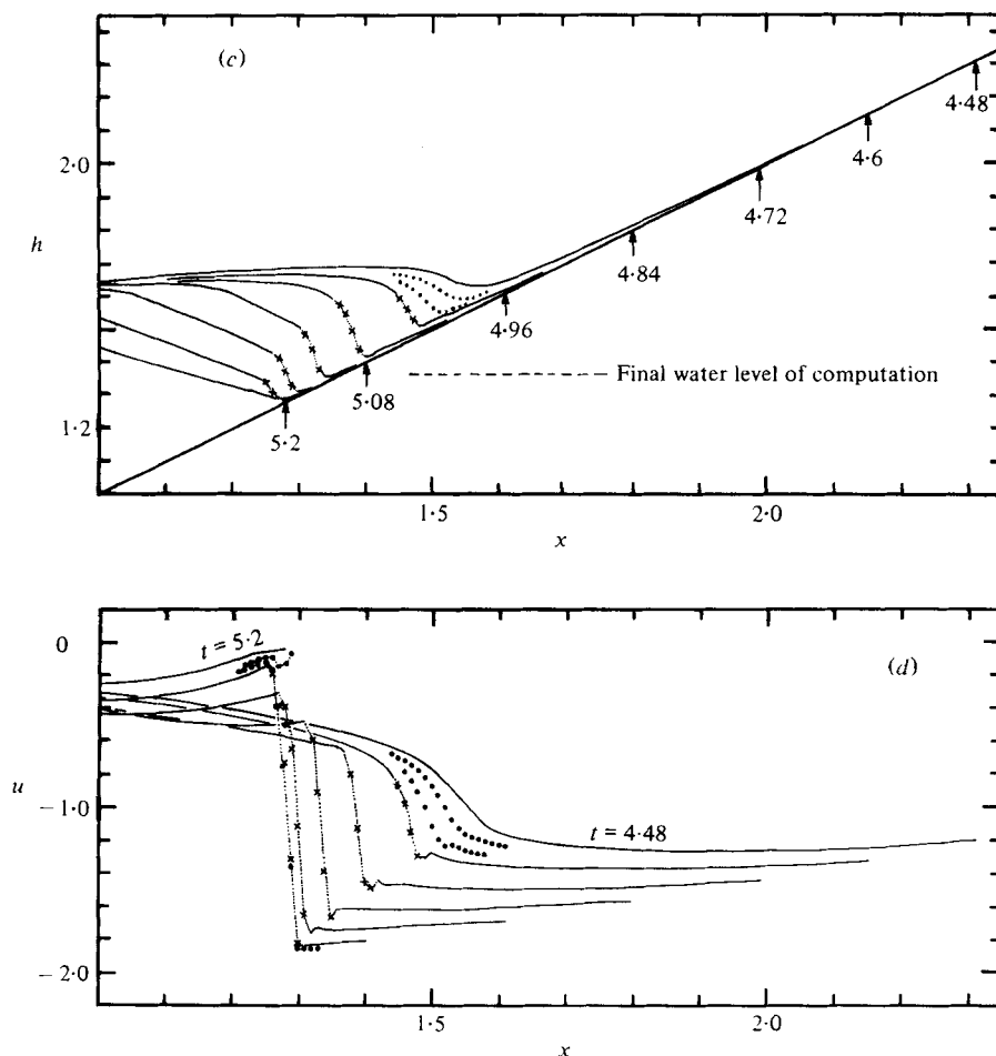
FIGURE 7. Computed solution for the backwash from a uniform bore of initial height = 1.6. (a) Surface elevation at t = 3.4 to 8.0 at intervals of 0.4. (b) Water velocity as in (a). (c) Detail of surface elevation for duration of the backwash bore, time intervals of 0.12, individual computation points are shown at the bore. Arrows indicate the shoreline position. (d) Detail of water velocity as in (c). Supplementary additional profiles are also shown.
