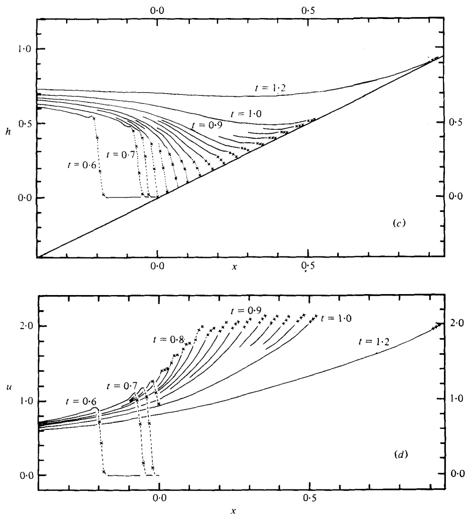
FIGURE 6. Computed solution for the run-up of a uniform bore. Initial bore height = 1.6. (a) Surface elevation at t = 0.4 to 3.2 at intervals of 0.4. (b) Water velocity, as in (a). (c) Detail of surface elevation, bore meeting the shoreline, time intervals of 0.02, individual computation points shown at the bore and the shoreline. (d) Detail of water velocity, as in (c). Supplementary additional profiles are also shown.
