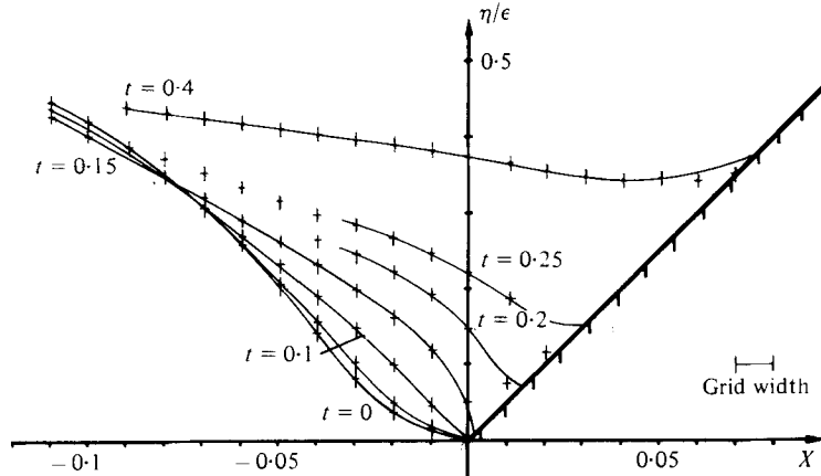
FIGURE 3. Comparison of present numerical scheme with the analytic solution of Carrier & Greenspan (1958) equation (3.1), \epsilon = 0.2 . + + +, present scheme; —, exact result.
