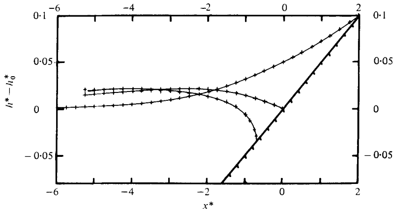
FIGURE 4. Comparison with the solution of Spielvogel (1976) for flow in the back-wash. —, result of Spielvogel ( R = 0.1 , H = 0.05 ); + + +, present scheme.
