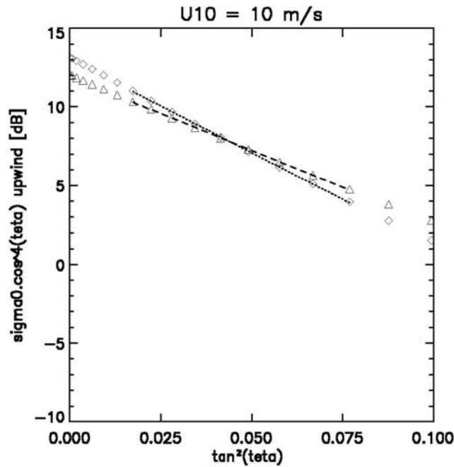
Figure 1. \sigma_0(\theta, \phi)\cos^4\theta (in dB) as a function of \tan^2\theta , as simulated by the Physical Optics model (see appendix A) and the sea surface spectrum given for a 10 m/s wind speed, by Elfouhaily et al. [1997] (diamonds) and Kudryavtsev et al. [2003] (triangles). The solid and dashed lines are the fit of equation (5) to the model results, applied in the incidence range [7-16^\circ] .
