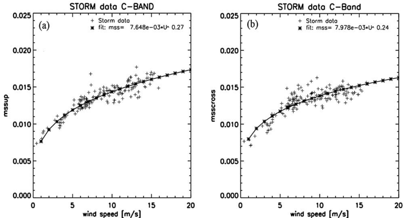
Figure 5. Mean square slope of the waves retrieved from the STORM observations in the incidence range 7\text{--}16^\circ , as a function of wind speed estimated from the STORM observations at 32.5^\circ incidence angle. (a) in the upwind direction (b) in the crosswind direction.
