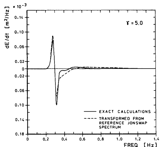
FIG. 3. Comparison of exact computations of one-dimensional S_{nl} distributions for JONSWAP spectra with \gamma = 1, 2 and 5 with parameterized form obtained by transforming from standard JONSWAP spectrum ( \gamma = 3.3 ).
