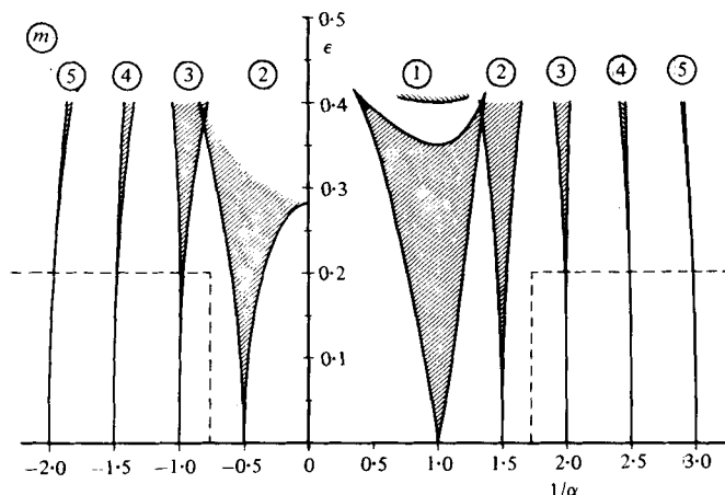
FIGURE 2. Stability diagram for perturbations of a Stokes wave (at \alpha = 1 ), negative values of \alpha^{-1} = \pm(|k_2|/k_1)^{\frac{1}{2}} corresponding to backward running waves. In the shaded area we have instability. The areas at m = 1 are taken from Longuet-Higgins (1978 b , figure 6). For m > 1 the stability diagram is qualitative at best outside of the area enclosed by the broken line, which marks the approximate limits of validity of our treatment. Further details are explained in the summary.
