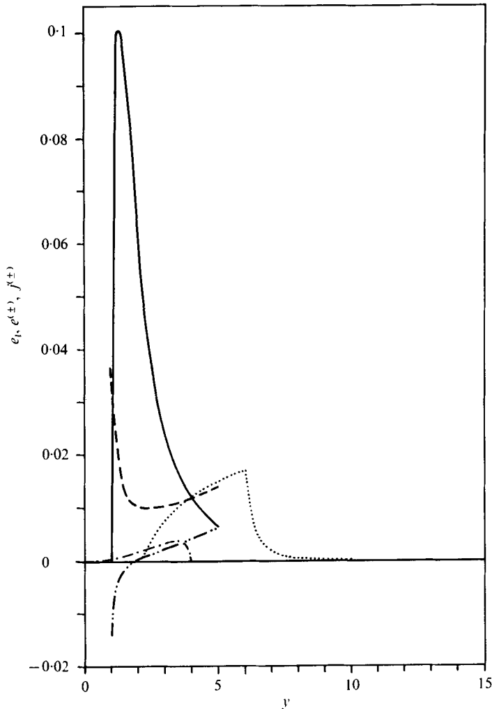
FIGURE 2. Normalized energy growth rates and fluxes for model A , calculated for wave spectrum (4.9) with \alpha = 0.01 , b = \sigma_c/\sigma_p = 5 and y_0 = c_{\text{peak}}/U = 1.0 . —, e_l , Snyder-Cox input; ----, e^{(+)} ; - · - ·, e^{(-)} ; · · · ·, j^{(+)} ; - - - -, j^{(-)} .
