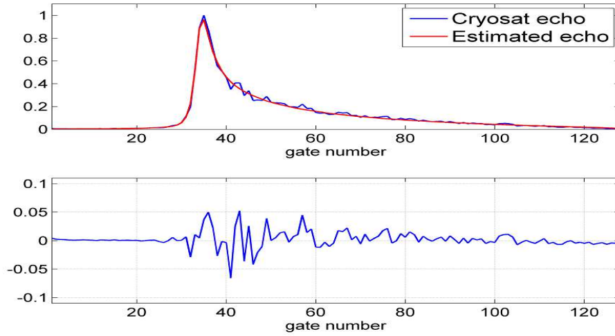
Figure 4.16: Estimated Cryosat-2 echo using the proposed DDA4 model ( \text{NRE} = 0.065 ). (top) real Cryosat-2 echo superimposed with its estimation, (bottom) difference between the real Cryosat-2 echo and its estimation.
