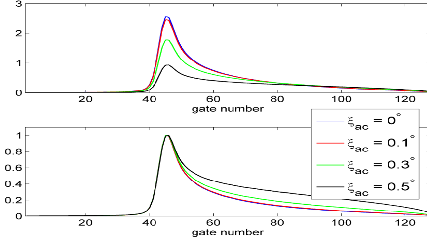
Figure 4.11: Effect of the across-track mispointing on (top) the multi-look echoes and (bottom) the normalized multi-look echoes (obtained with P_u = 1 , \tau = 44 gates, \text{SWH} = 3 meters and \xi_{\text{al}} = 0^\circ ).
