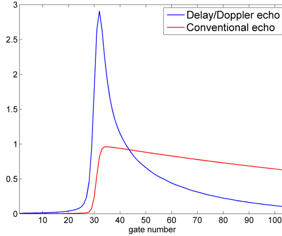
Figure 3.8: Delay/Doppler and conventional echoes for the same altimetric parameters ( P_u = 1 , \tau = 31 gates, SWH = 2 m).
