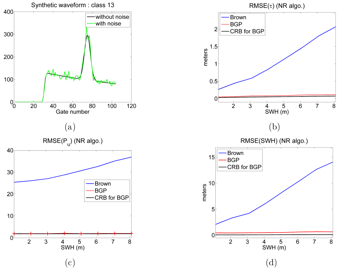
Figure 2.8: Parameter RMSEs for waveforms of class 13 with NR algorithm when using Brown (blue) and BGP (red) models. The CRBs of the BGP model parameters are also shown (black) for comparison.
