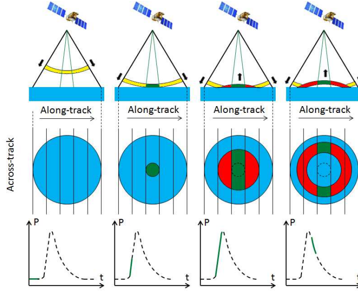
Figure 1.8: Formation of the central beam DDA waveform.
