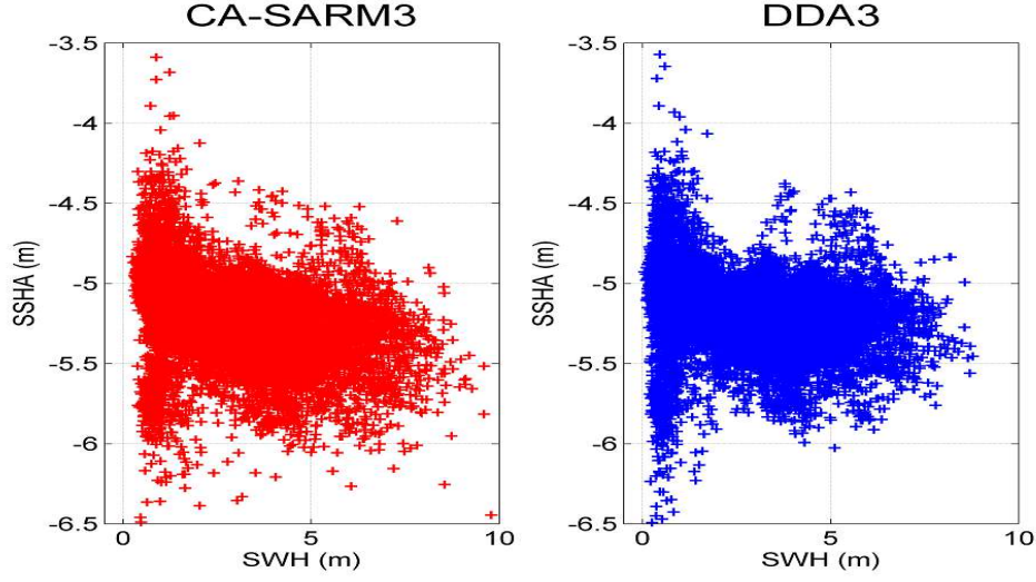
Figure 3.19: Correlations between estimated SWH and SSHA parameters for CA-SARM3 (left) and DDA3 (right).
