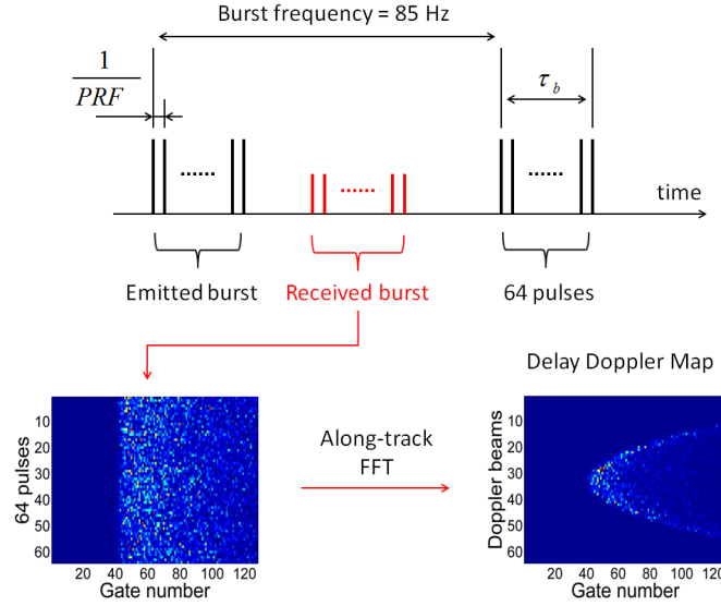
Figure 3.1: Configuration of a delay/Doppler altimeter and construction of a delay/Doppler map.
