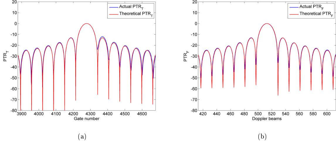
Figure 3.5: Temporal and frequency radar system point target response. (a) Actual Cryosat-2 PTR_T and the theoretical one, (b) actual Cryosat-2 PTR_F and the theoretical one.
