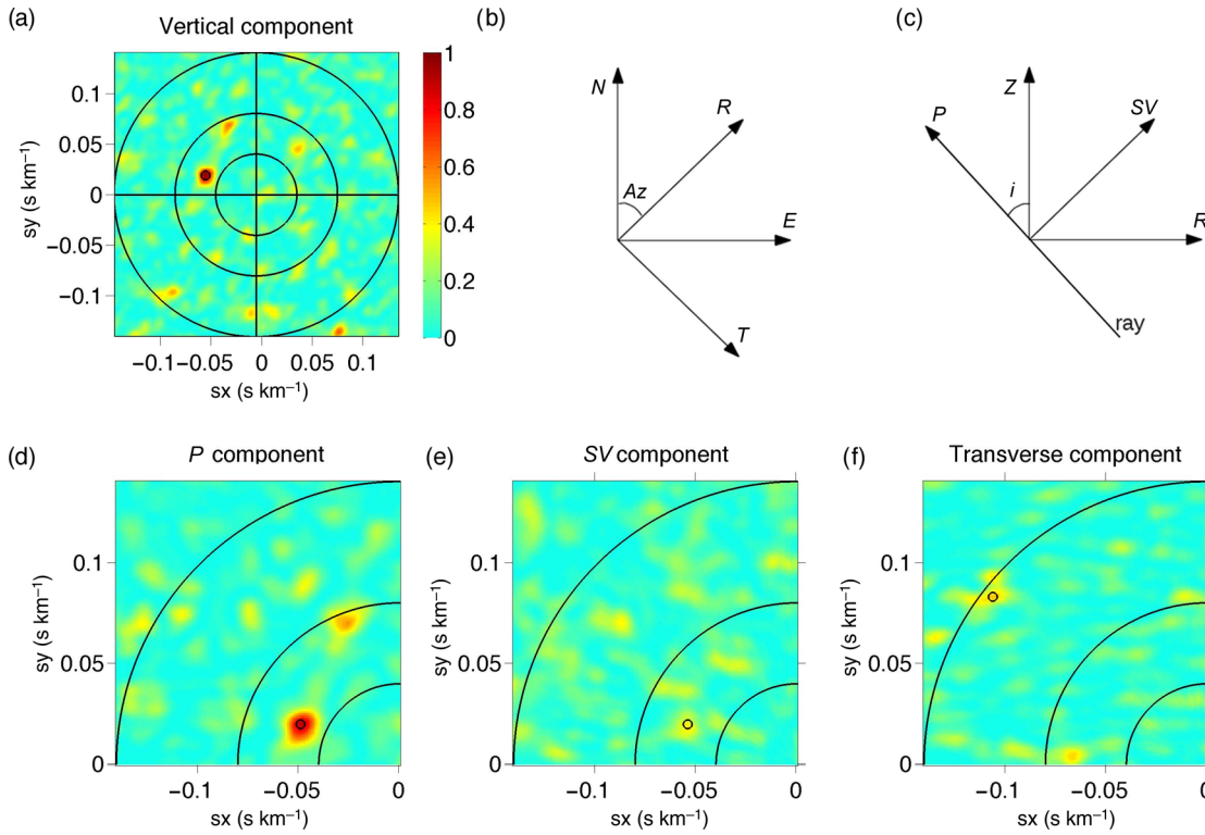
Figure 6. (a) Beamforming power spectrum of the vertical component seismograms. The colour scale is normalized to the vertical component maximum. (b), (c) Cartoon of the coordinates. The Z-axis is vertical and the R-axis is horizontal towards the network-source azimuth. The P and SV-axes are in the vertical plane defined by Z and R. The P-axis is towards the theoretical direction of the incident P wave, and the SV-axis is perpendicular to P. The P-component (d), SV-component (e) and T-component (f) beamforming power spectra. The small black circles indicate the beam maximum. The large black circles and circle arcs correspond to slownesses of 0.04, 0.08 and 0.14 s km -1 . For a distance range of 30° to 90°, the P-wave slowness is between 0.04 and 0.08 s km -1 , and the S-wave slowness is between 0.08 and 0.14 s km -1 .
