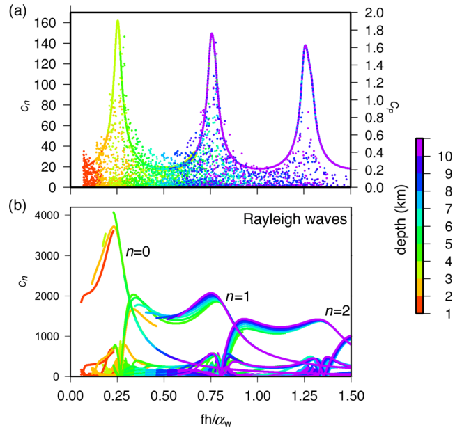
Figure A1. (a) Comparison between the results obtained using normal modes (dots) and the plane wave superposition approach (solid line) for epicentral distances between 30° and 90°. The amplitude of c_n (normal-modes approach) is shown on the left and the amplitude of c_P (plane wave superposition approach) on the right. The ocean depth is shown in colour. For computing the P -wave site effect using normal modes, it is necessary to integrate all of the contributions shown in this figure (dots), with each one multiplied by a phase. Small differences are due to the different earth models (PREM model with normal modes and an ocean layer over a half-space for the plane wave superposition approach). (b) Rayleigh wave site effect computed using normal modes (modified from Gualtieri et al. 2013).
