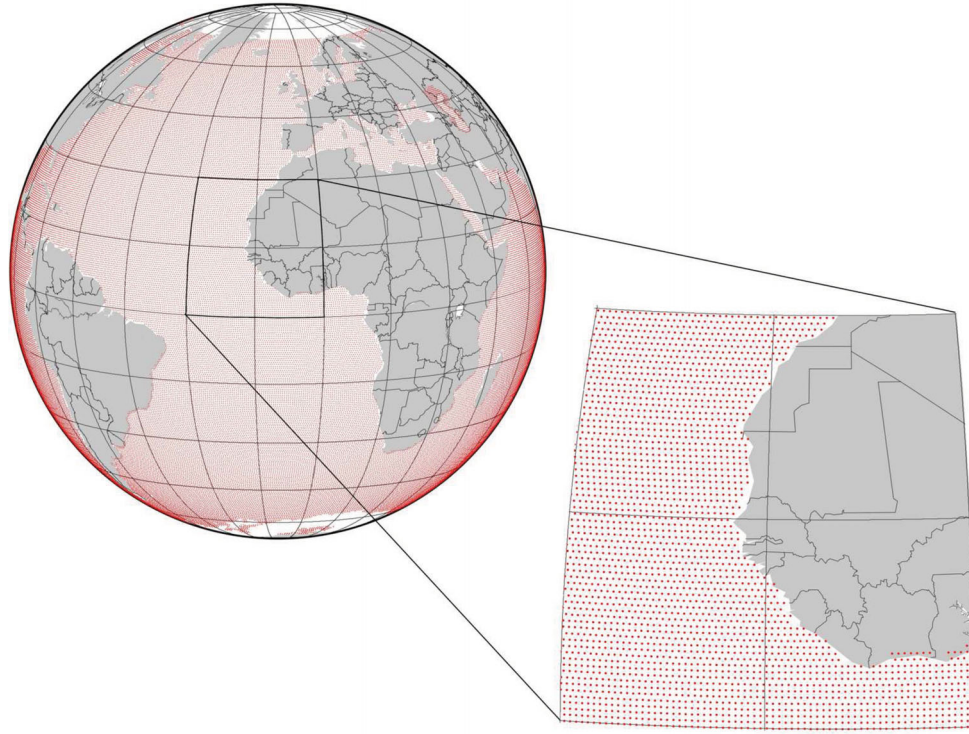
Figure 1. Spherical grid of noise point sources. All the ocean is discretized with a step of 50 km. This represents a good compromise between solution convergence and calculation time.
