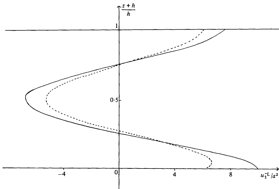
FIGURE 3. A plot of \bar{u}_2^{-L} as a function of z , for \kappa = \frac{1}{2}\pi , when V = 0.23 , c_{2m}^{(0)} = 0.16 ; — T = 1 and X = 0.2 , --- T = 2 and X = 0.4 . We have set N = 1 , h = 1 , m = 1 and E = \epsilon^2 = 10^{-4} .
