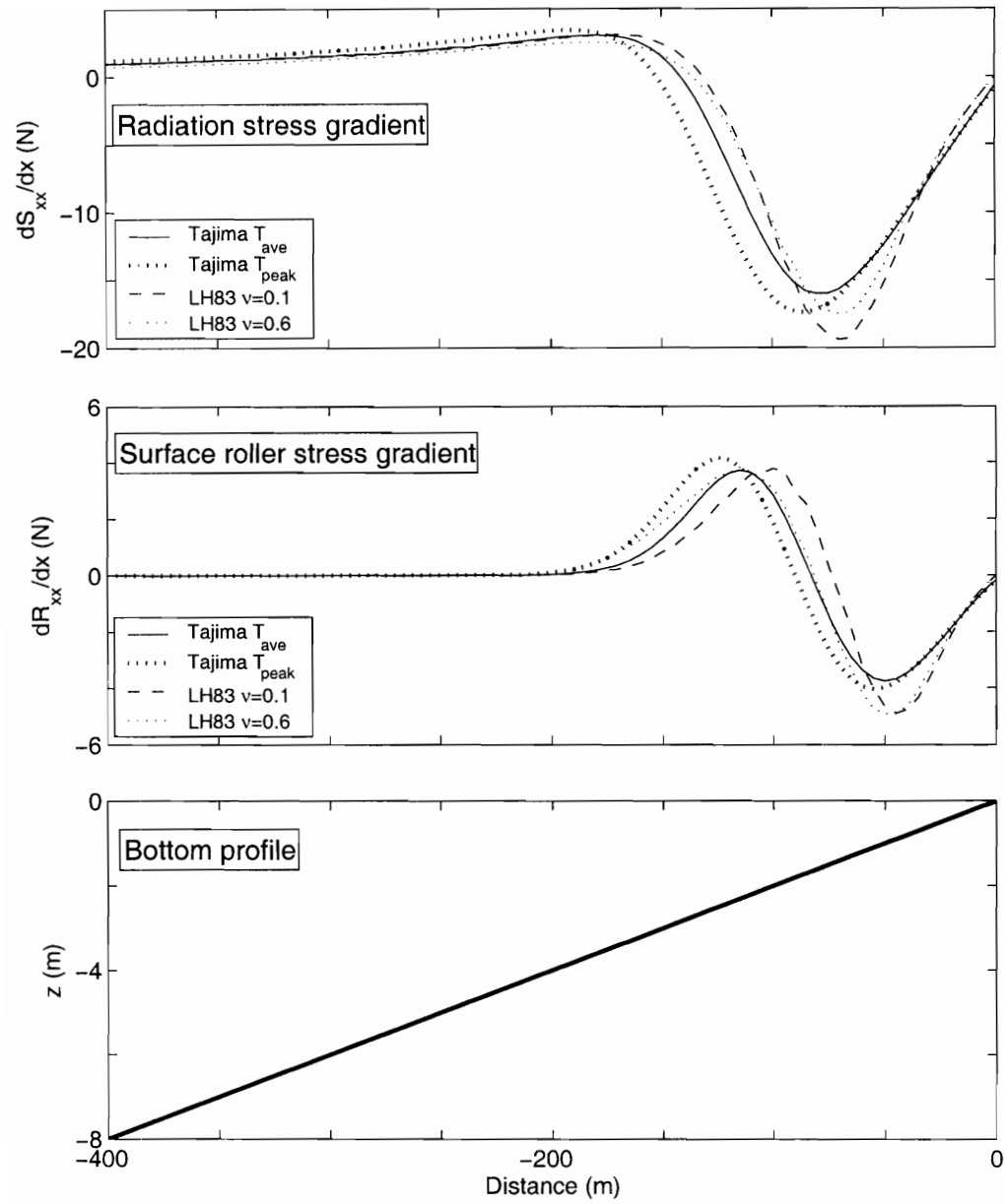
Figure 3-3: Comparison of radiation stress gradients and surface roller stress gradients in the plane beach case. Tajima's spectral model for H_{rms} and T_{ave} (solid line), Tajima's spectral model for H_{rms} and T_{peak} (thick dotted line), and Longuet-Higgins's (1983) distribution, for \nu = 0.1 (dashed line) and \nu = 0.6 (thin dotted line). Different wave period durations are not accounted for when averaging.
