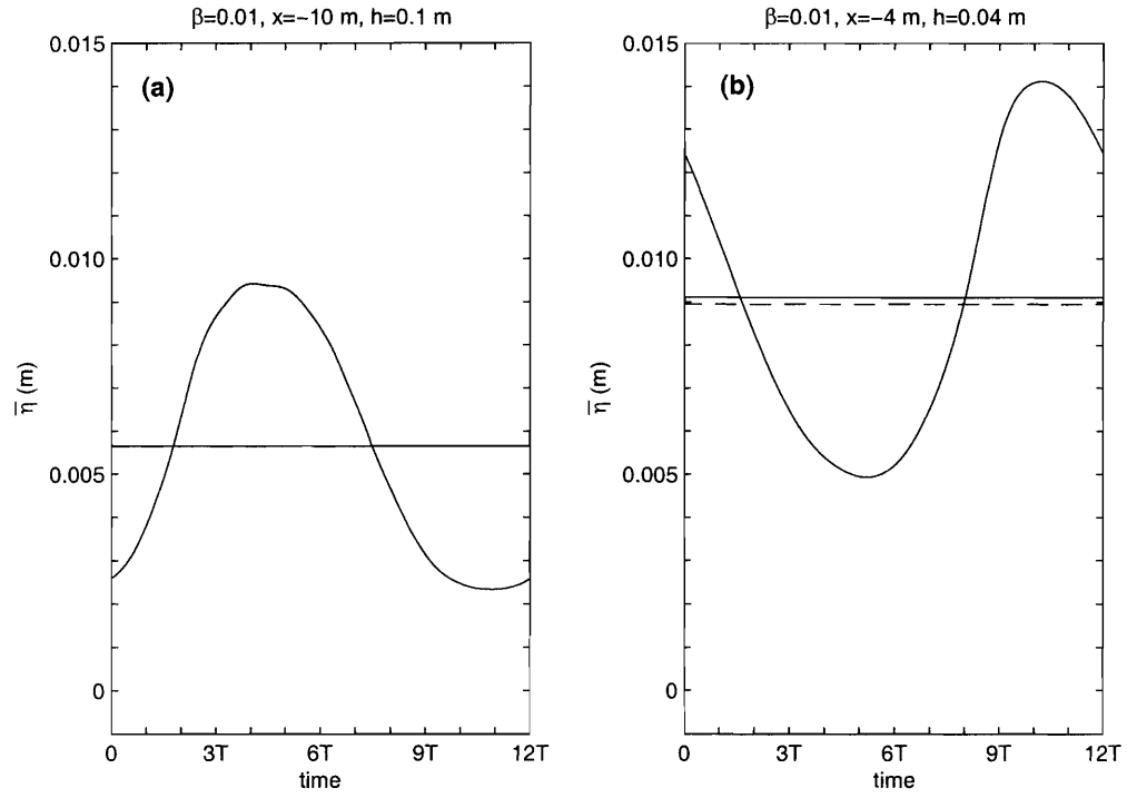
Figure 4-9: Mean wave set-up evolution over the wave beat in a plane beach of mild slope, \tan \beta = 0.01 , at specific cross-shore locations: (a) x = -10 m; (b) x = -4 m. The horizontal solid line represents the time-average value and the horizontal dashed line is Tajima's steady monochromatic model solution.
