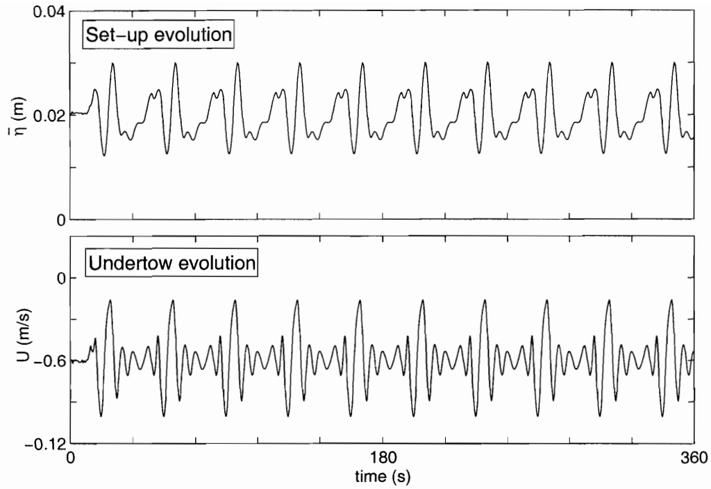
Figure 4-4: Evolution of the mean wave set-up ( \bar{\eta} ) and undertow ( U ) at x = -0.8 m. Periodicity is achieved quickly.
