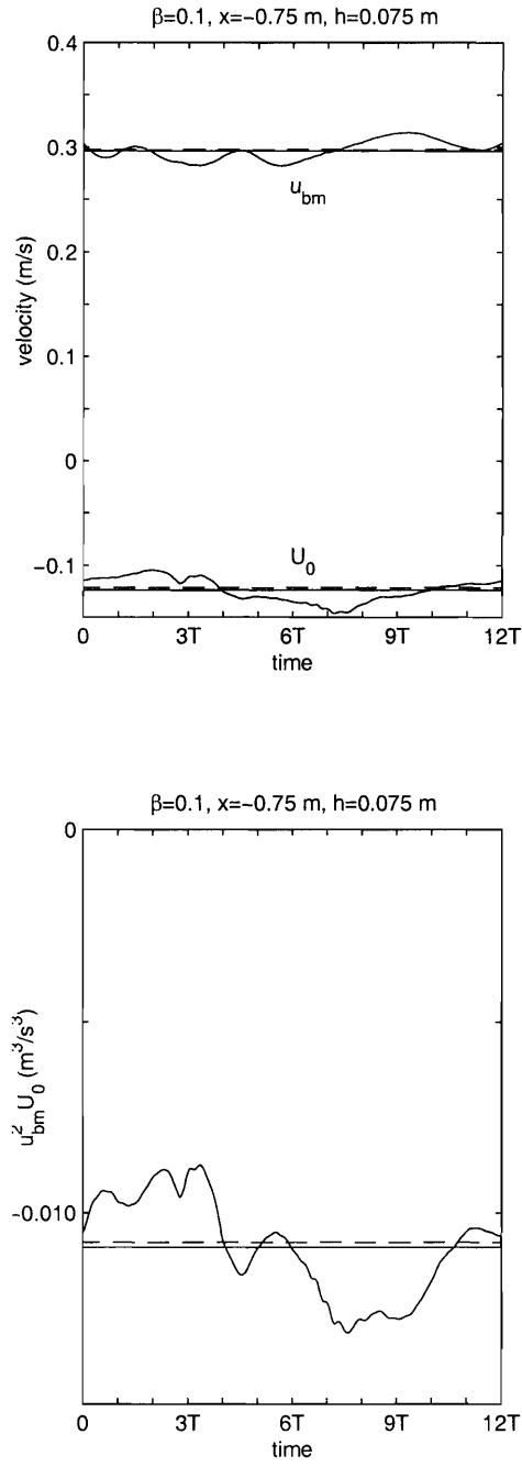
Figure 4-11: Wave bottom orbital velocity, undertow, and estimation of sediment transport for a plane beach of slope \tan \beta = 0.1 at x = -0.75 m. Horizontal solid lines represent time-average values and horizontal dashed lines are Tajima's steady monochromatic model solutions.
