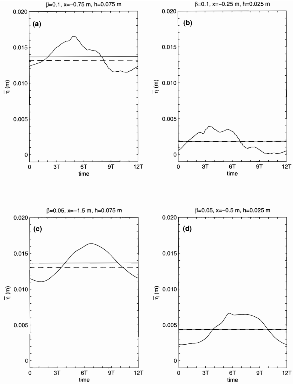
Figure 4-7: Mean wave set-up evolution over the wave beat in plane beaches of steep slope at specific cross-shore locations: (a) \tan \beta = 0.1 , x = -0.75 m; (b) \tan \beta = 0.1 , x = -0.25 m; (c) \tan \beta = 0.05 , x = -1.5 m; (d) \tan \beta = 0.05 , x = -0.5 m. The horizontal solid line represents the time-average value and the horizontal dashed line is Tajima's steady monochromatic model solution.
