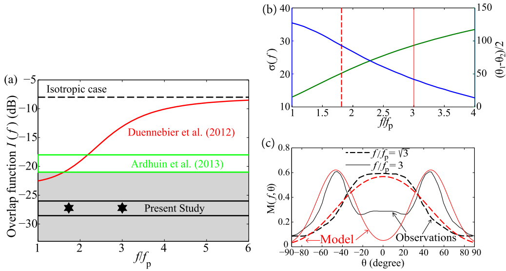
Fig. 10. Directional properties of the OSGWs associated with our average inverted I -value of -27 dB. (a) I -values inverted in our study as compared to those inverted from acoustic noise in the previous studies of Duennebier et al. (2012) and Ardhuin et al. (2013). These studies both inverted I at ALOHA, i.e. for similar 2 to 16 m/s wind speeds, and I -values have been taken in a similar frequency range (0.5 to 1.5 Hz). The grey region indicates the range of possible I -values including all model uncertainties. Black stars indicate the configurations shown in Fig. 10(c). (b) Standard deviation \sigma(f) (blue line) and angle difference (\theta_1 - \theta_2)/2 (green line) associated with the double-Gaussian formulation of equation (19). The angle difference (\theta_1 - \theta_2)/2 is set from the formulation of Ewans (1998) (see equation (20)), while \sigma(f) is inverted such that our average value of I = -27 dB is obtained (see Fig. 10(a)). Vertical dashed and dotted lines indicate the configurations shown in (c). (c) Directional function M(f, \theta) as a function of \theta for frequencies f = \sqrt{3}f_p (dashed lines) and f = 3f_p (continuous lines) as inverted in this study (red) and as observed by Hwang et al. (2000) (black). (For interpretation of the references to color in this figure legend, the reader is referred to the web version of this article.)
