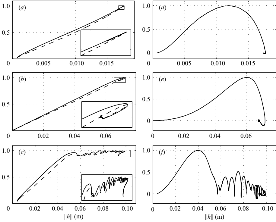
FIGURE 16. H_{rms} = 1.0 m, T = 6 s. (a–c) Square root of the —, production and ---, damping terms as a function of \|h\| . (d–f) Difference between production and damping, (\mathcal{P} + \Delta) as a function of \|h\| . (a, d) SVR transport, \theta = 0^\circ , (b, e) SVR transport, \theta = 25^\circ , (c, f) CWS transport, \theta = 25^\circ .
