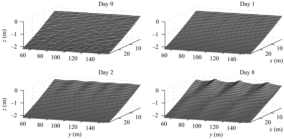
FIGURE 4. SVR transport, H_{rms} = 1.0 m, T = 6 s, \theta = 0^\circ . Zoom of the total bathymetry during the formation, development and growth saturation of shore-transverse bars.
