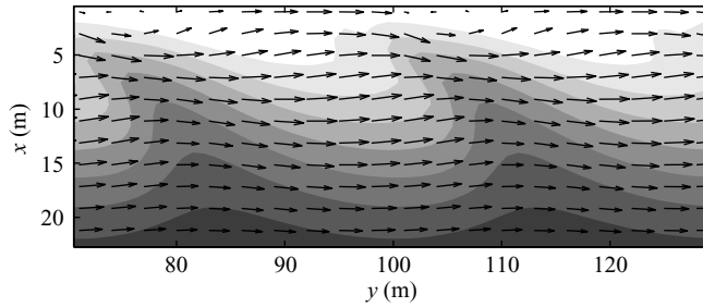
FIGURE 8. SVR transport, H_{rms} = 1.0 m, T = 6 s, \theta = 25^\circ . Final state (day 14). Bathymetric contours ( z_b ) and circulation ( v ) over down-current oriented bars. Shallowest areas are white and deepest areas are shaded.
