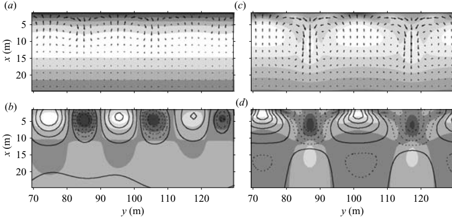
FIGURE 13. SVR transport, H_{rms} = 1.0 m, T = 6 s, \theta = 0^\circ . Left (a, b) Initial state (day 3). (c, d) Final state (day 12). (a, c) \alpha/D (small values are shaded and large values are white) and current vectors. (b, d) D\mathbf{v} \cdot \nabla(\alpha/D) (negative values (accretion) are white and positive values (erosion) are shaded) and bottom perturbation ( h ) contours (crests are straight lines, troughs are dotted lines).
