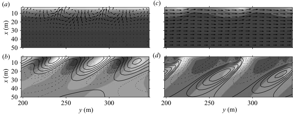
FIGURE 15. CWS transport, H_{rms} = 1.0 m, T = 6 s, \theta = 25^\circ . (a, b) Initial state (day 5). (c, d) Final state (day 85). The graph description is the same as figure 14.
