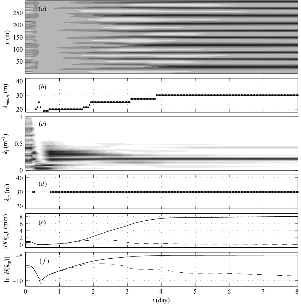
FIGURE 6. SVR transport, H_{rms} = 1.0 m, T = 6 s, \theta = 0^\circ . Time series of (a) the bed level along the longshore section at x = 10 m ( h(y, t) ), crests are white and troughs are black, (b) the mean spacing of the bars ( \lambda_{mean}(t) ), (c) the normalized modulus of the Fourier coefficient of the topographic signal ( |\mathcal{H}|_n(k_l, t) ), (d) the resulting predominant spacing of bars ( \lambda_m(t) ), (e) the two predominant most energetic (non-normalized) Fourier coefficients of the topographic signal ( |\mathcal{H}|(k_l, t) ), corresponding to: \lambda_m = 2\pi/k_m = 20 m (dashed line), \lambda_m = 30 m (thick line), and (f) their logarithmic value ( \ln |\mathcal{H}(k_m, t)| ).
