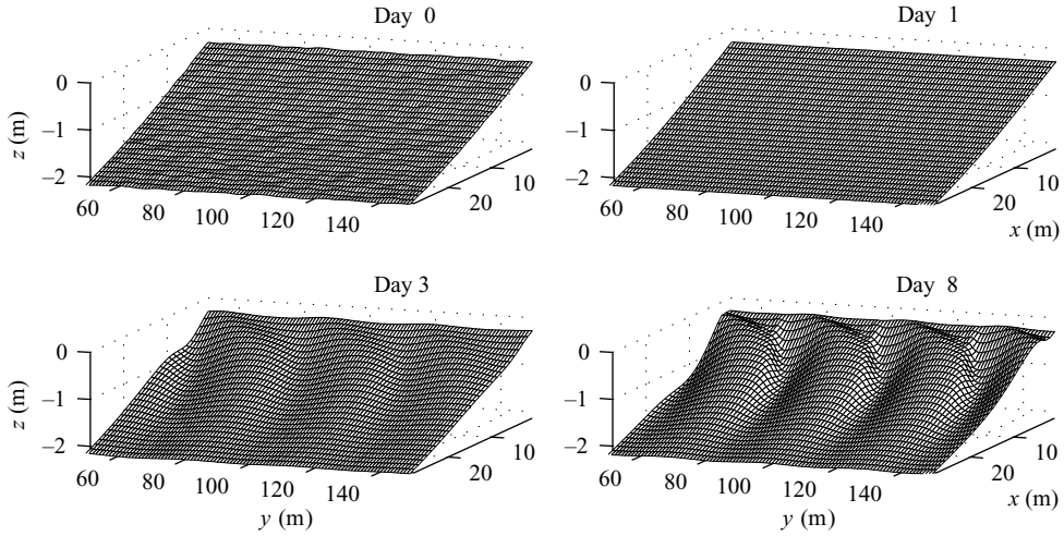
FIGURE 7. SVR transport, H_{rms} = 1.0 m, T = 6 s, \theta = 25^\circ . Zoom of the total bathymetry during the formation, development and growth saturation of oblique down-current oriented bars.
