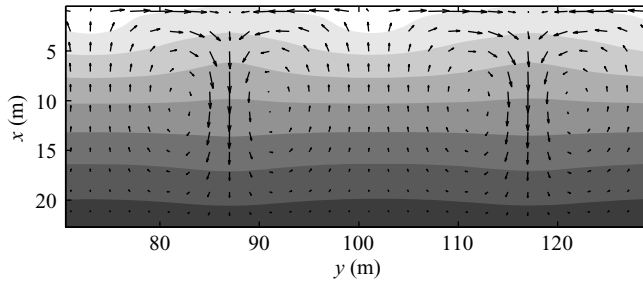
FIGURE 5. SVR transport, H_{rms} = 1.0 m, T = 6 s, \theta = 0^\circ . Final state (day 8). Bathymetric contours ( z_b ) and circulation ( v ) over transverse bars. Shallowest areas are white and deepest areas are shaded.
