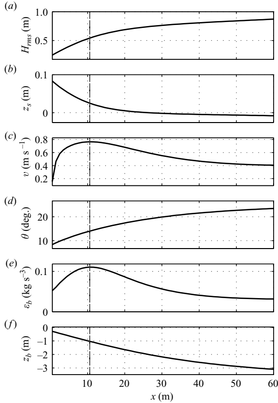
FIGURE 2. H_{rms} = 1.0 m, T = 6 s, \theta = 25^\circ . Equilibrium profiles of the basic state in the case of oblique wave incidence. (a) Wave height ( H_{rms} ), (b) mean sea level ( z_s ), (c) longshore velocity ( v ), (d) wave angle ( \theta ), (e) dissipation rate ( \epsilon_b ) and (f) bottom level ( z_b ). Shoreline at x = 0 .
