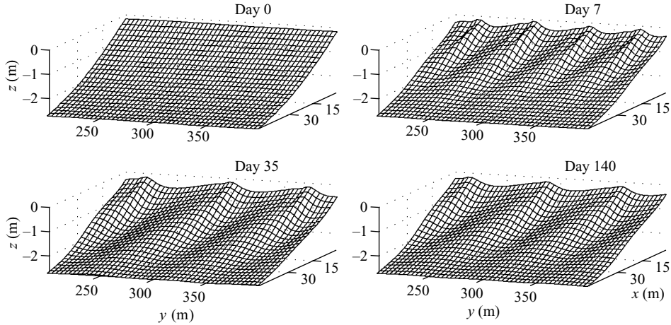
FIGURE 10. CWS transport, H_{rms} = 1.0 m, T = 6 s, \theta = 25^\circ . Zoom of the total bathymetry during the formation, development and growth saturation of oblique up-current oriented bars.
