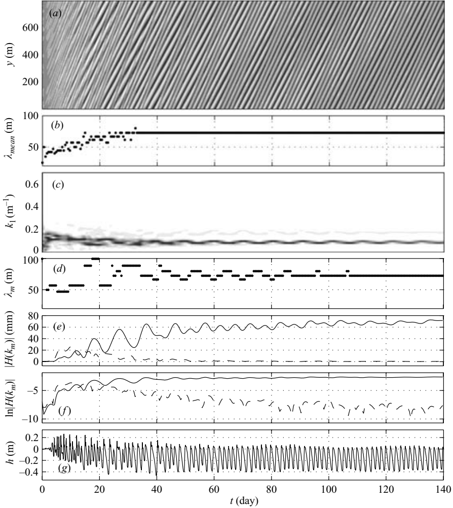
FIGURE 12. CWS transport, H_{rms} = 1.0 m, T = 6 s, \theta = 25^\circ . The graph description is the same as figure 9 but for (e) and (f), \lambda_m = 2\pi/k_m = 50 m (dashed line), \lambda_m = 72 m (thick line).
