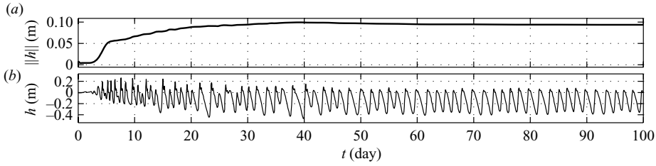
FIGURE 18. CWS transport, H_{rms} = 1.0 m, T = 6 s, \theta = 25^\circ . Time evolution of (a) \|h\| and (b) h(10, 22.5) .
