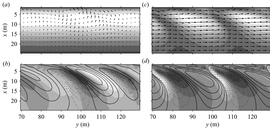
FIGURE 14. SVR transport, H_{rms} = 1.0 m, T = 6 s, \theta = 25^\circ . (a, b) Initial state (day 8). (c, d) Final state (day 14). The graph description is the same as figure 13, but vectors in (a) show only the current perturbation.
