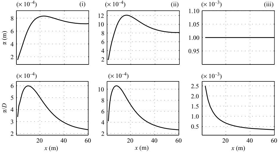
FIGURE 3. H_{rms} = 1.0 m, T = 6 s. Stirring factor \alpha (up) and potential stirring \alpha/D (down) at the equilibrium state for three cases: (i) SVR transport, \theta = 0^\circ , (ii) SVR transport, \theta = 25^\circ , (iii) CWS transport, \theta = 25^\circ .
