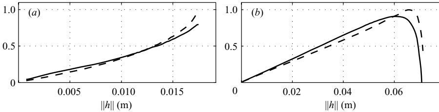
FIGURE 17. SVR transport, H_{rms} = 1.0 m, T = 6 s. Derivatives of —, d\mathcal{P}/d\|h\| and ---, -d\Delta/d\|h\| as a function of \|h\| . (a) \theta = 0^\circ , (b) \theta = 25^\circ .
