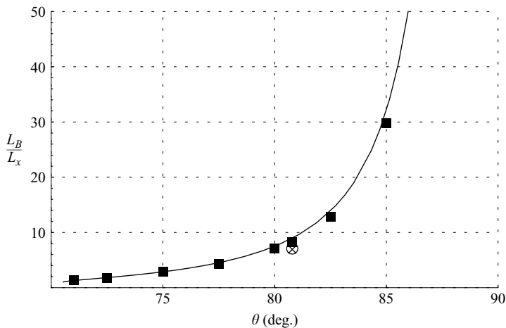
FIGURE 7. Comparison of the theoretical (line, from (4.14)) and computed (squares) beat length of the first harmonic amplitude. The computed points are from simulations with steepness ak=0.15 , except for the case with \theta=85^\circ where ak=0.10 . The additional \circ marks the computed beat length for case C14 (with ak=0.40 ) from figure 5(c), while \times marks the corresponding experimental value estimated from figure 11(a) (bottom sub-figure) of Hammack et al. (2005).
