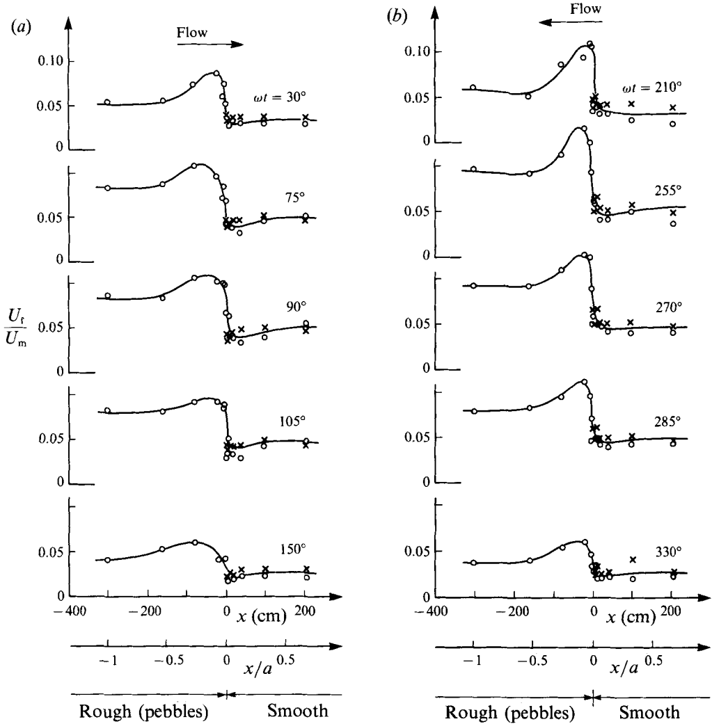
FIGURE 7. Time evolution of bed shear velocity, \circ , logarithmic fit. \times , direct measurements. Test series 1.
