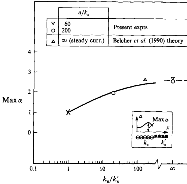
FIGURE 10. Maximum amplification factor regarding the bed shear stress. ○, test series 1 and 3. ∇, test series 2. ×, the case where the bed has a uniform roughness.
