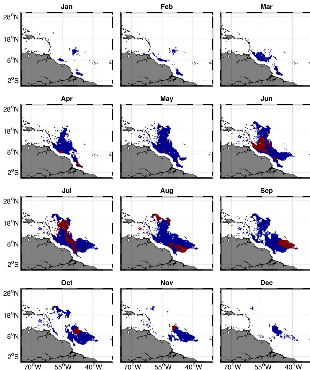
Figure 4. Seasonal evolution of the Amazon plume extension. Every month, the 0.25 \times 0.25^\circ pixels reached by the plume (months during which the a_{\text{cdm}} peak occurs for each pixel) are colored in blue. The pixels for which the time series extrema occurs in the current month are colored in red.
