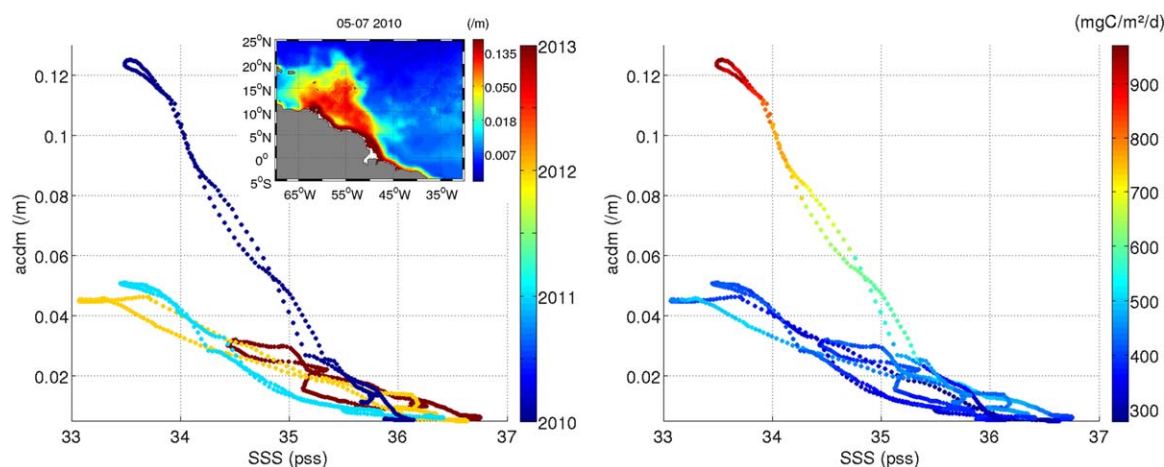
Figure 15. The 25 km 90 day a_{\text{cdm}} versus SMOS SSS at location 3 ( 14^{\circ}\text{N} , 55^{\circ}\text{W} ) pointed out by a black dot on the May through July average a_{\text{cdm}} map. The z axis represents (left) the year of observation and (right) the CbPM net primary productivity from Ocean Productivity.
