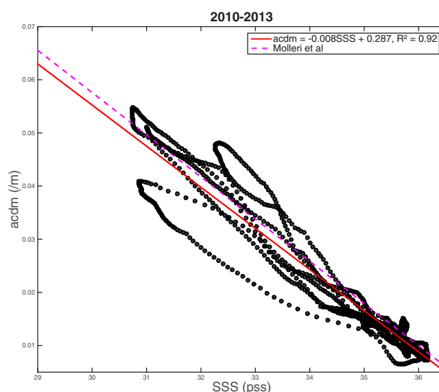
Figure 6. The 25 km 90 day running mean a_{\text{cdm}} as a function of 25 km 90 day running mean SMOS SSS over 2010–2013 (black dots) at location 1 shown in Figure 2. The red solid line represents the linear regression computed for that pixel over 2010–2013. The magenta dotted line represents the Moller et al. [2010] linear model.
