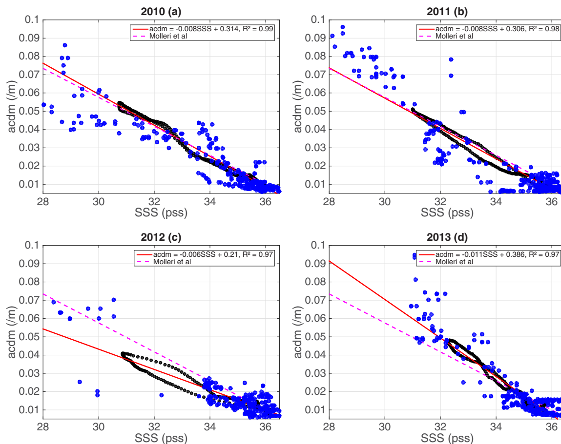
Figure 7. The 25 km 90 day running mean a_{\text{cdm}} as a function of 25 km 90 day running mean SMOS SSS in (a) 2010, (b) 2011, (c) 2012, and (d) 2013 (black dots) at location 1 shown in Figure 2. The red solid line represents the linear regression computed for that pixel for each year. The magenta dotted line represents the Moller et al. [2010] linear model. The blue dots represent the 25 km 10 day running mean a_{\text{cdm}} as a function of 25 km 90 day running mean SMOS SSS in each year.
