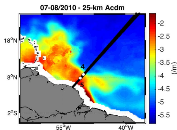
Figure 12. Average July to August 2010 a_{\text{cdm}} map on top of which are represented as solid black lines, three TSG transects. The white dots, labeled 4 and 5, mark the locations [7.75°N 50.75°W] and [8.75°N 50°W].
