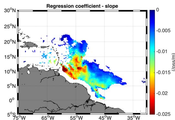
Figure 8. Slope of the linear regression between the time series of filtered SMOS SSS and a_{\text{cdm}} for each 0.25 \times 0.25^\circ pixel over 2010–2013. Only pixels in the plume for which the p -value (significance of the SSS- a_{\text{cdm}} correlation) is below 0.01 and time lag between the SMOS SSS minimum and a_{\text{cdm}} maximum is zero are shown.
