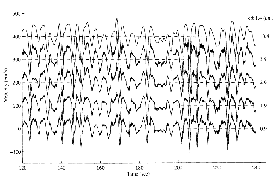
Figure 5. A 2 min time series of the derectified calibrated velocity as measured by fur hot film anemometers within the wave bottom boundary layer and in the free stream as measured by an EMC. The average distance of each sensor from the bed as measured by the FOBS over the 2 min record is listed at right. Each time series is offset from the others by 100 cm/s. Onshore directed flow is indicated with negative velocities, and offshore flow is indicated with positive velocities.
