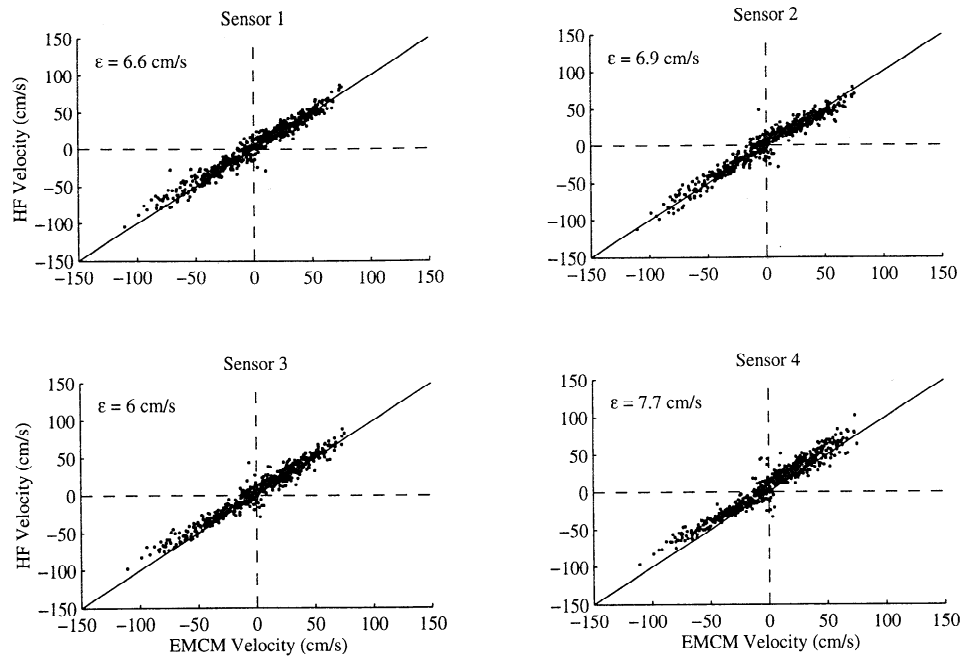
Figure 3. Comparison of the cross-shore velocities as measured by the electromagnetic current meter (ECM) and the calibrated, derectified cross-shore velocities as measured by hot film sensors (HF1-HF4). Each record has been digitally low-pass filtered to 1 Hz. The rms deviation, \varepsilon , between the ECM and each HF is specified for each comparison.
