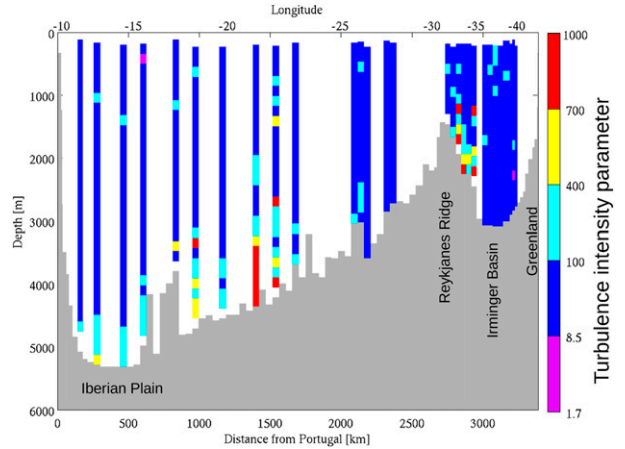
FIG. 6. Turbulence intensity parameter \text{Re}_b = \varepsilon/(\nu N^2) . The color scale is nonlinear and emphasizes four mixing regimes (bounded by 1.7, 8.5, 400).
