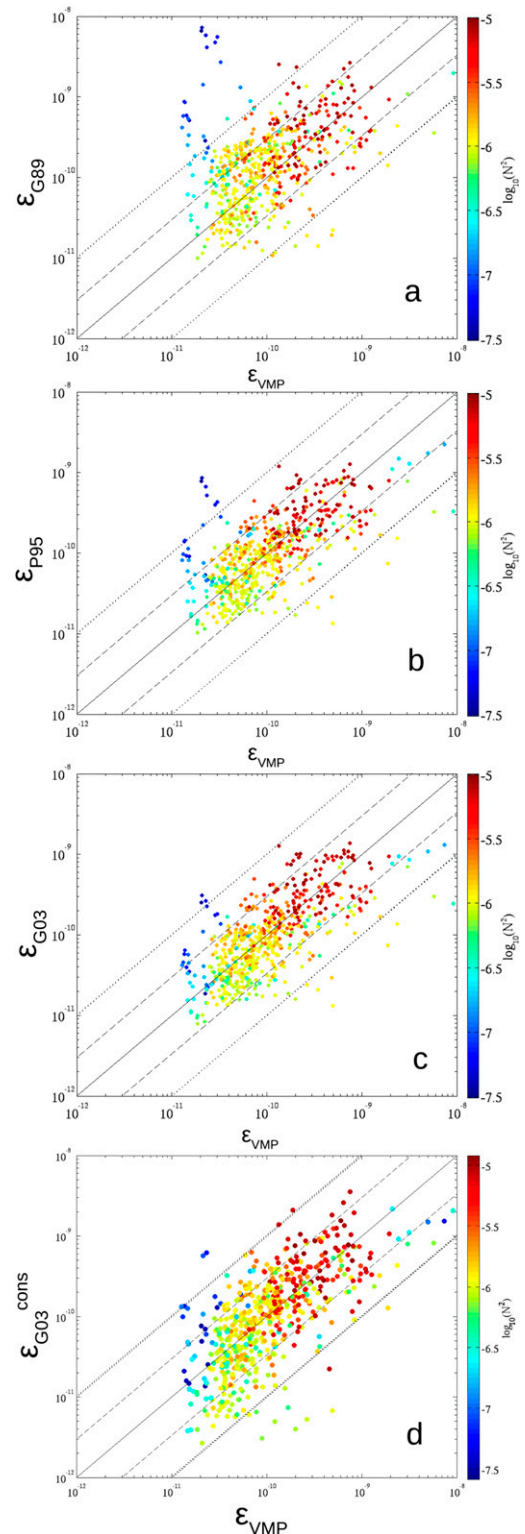
FIG. 7. Dissipation rate \varepsilon_{\text{finestructure}} as a function of \varepsilon_{vmp} . (a)–(d) Color scale denotes \log_{10}(N^2) with \varepsilon_{\text{finestructure}} = \varepsilon_{G89}, \varepsilon_{P95}, \varepsilon_{G03}, \varepsilon_{G03}^{\text{cons}} , respectively. Solid line denotes perfect agreement with microstructure, dashed lines represent a factor of 3, and dotted lines represent a factor of 10.
