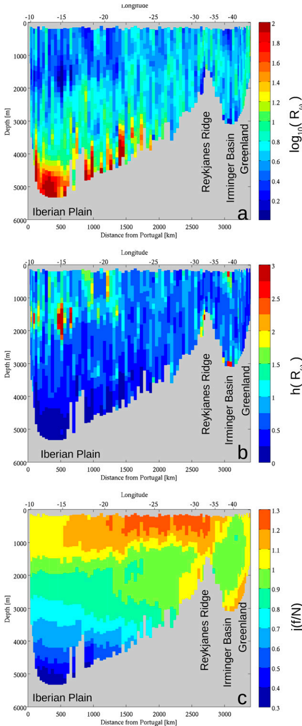
FIG. 8. (a) Shear-to-strain ratio R_\omega , (b) frequency modulation term h(R_\omega) , and (c) latitude/buoyancy frequency modulation term j(f/N) used in the finescale parameterizations \varepsilon_{P95} and \varepsilon_{G03} .
