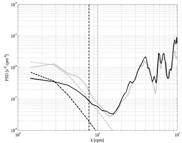
FIG. 2. Example of an average of four PSD of microstructure velocity shear (solid) observed with the VMP for the profile located at 42^{\circ}35'N , 15^{\circ}27'W and at a depth of 4200 (gray) and 4270 m (black). Dashed curves are matching Nasmyth (1970) spectra for \varepsilon = 7.2 \times 10^{-11} \text{ W kg}^{-1} (gray) and for \varepsilon = 2.6 \times 10^{-11} \text{ W kg}^{-1} (black). Vertical lines give the corresponding Kolmogorov wavenumber.
