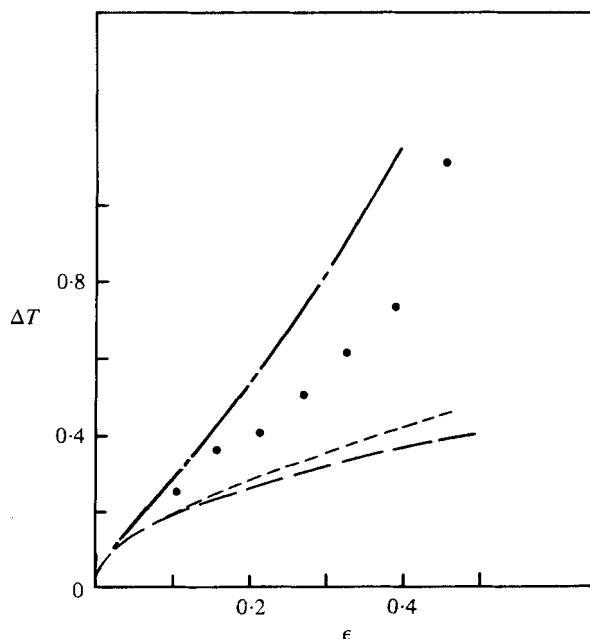
FIGURE 11. Time phase lag at the wall. ●, measured in the present work; —, second-order theory; — — —, third-order immediate post-interaction; — · — · —, third-order long-term.
