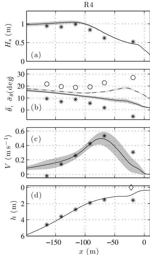
Figure 8. Modeled (curves) and observed (symbols) (a) H_s , (b) \bar{\theta} (solid and asterisks) and \bar{\sigma}_\theta (dashed and circles), (c) V , and (d) depth h versus x for R4. See Figure 5 caption for details.
