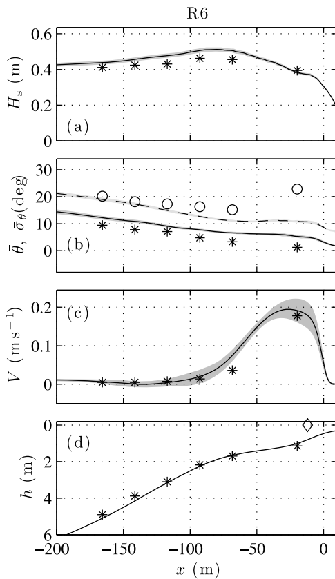
Figure 9. Modeled (curves) and observed (symbols) (a) H_s , (b) \bar{\theta} (solid and asterisks) and \bar{\sigma}_\theta (dashed and circles), (c) V , and (d) depth h versus x for R6. See Figure 5 caption for details.
