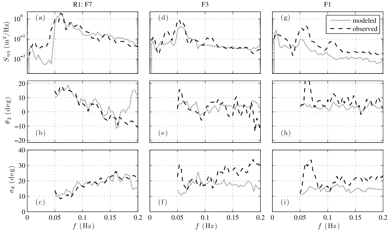
Figure 10. Release R1 (a, d, and g) sea surface elevation spectra S_{\eta\eta} , (b, e, and h) wave angle \theta_2 , and (c, f, and i) directional spread \sigma_\theta versus f for seaward of the surf zone at F7 (Figures 10a–10c), mid surf zone at F3 (Figures 10d–10f), and near-shoreline at F1 (Figures 10g–10i). In Figures 10b, 10e, and 10h, the black dashed line represents \theta_2 = 0^\circ . Note that \theta_2(f) and \sigma_\theta(f) are only estimated at sea swell frequencies ( 0.05 < f < 0.2 Hz).
