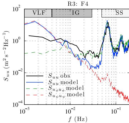
Figure 13. Release R3 cross-shore velocity spectra S_{uu} versus frequency f in the surf zone at F4. Observed (solid black), model (solid blue), irrotational model ( S_{u_\phi u_\phi} , green dashed), and rotational model ( S_{u_\psi u_\psi} , red dashed) spectra are indicated in the legend. The VLF ( 0.001 < f < 0.004 Hz), IG ( 0.004 < f < 0.03 Hz), and SS ( 0.05 < f < 0.2 Hz) frequency bands are indicated by the shaded regions at the top.
