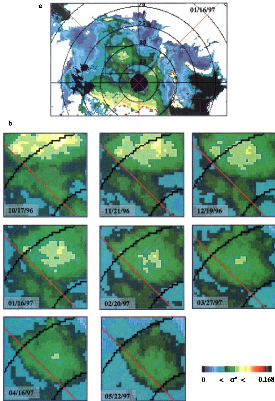
Plate 2. Weekly active microwave instrument operating in wind mode (AMI-Wind) backscatter map at 40^\circ incidence angle centered on January 16, 1997, showing (a) the area studied, with the square indicating the area zoomed, and (b) time series of the zooms from October 17, 1996, to May 22, 1997.
