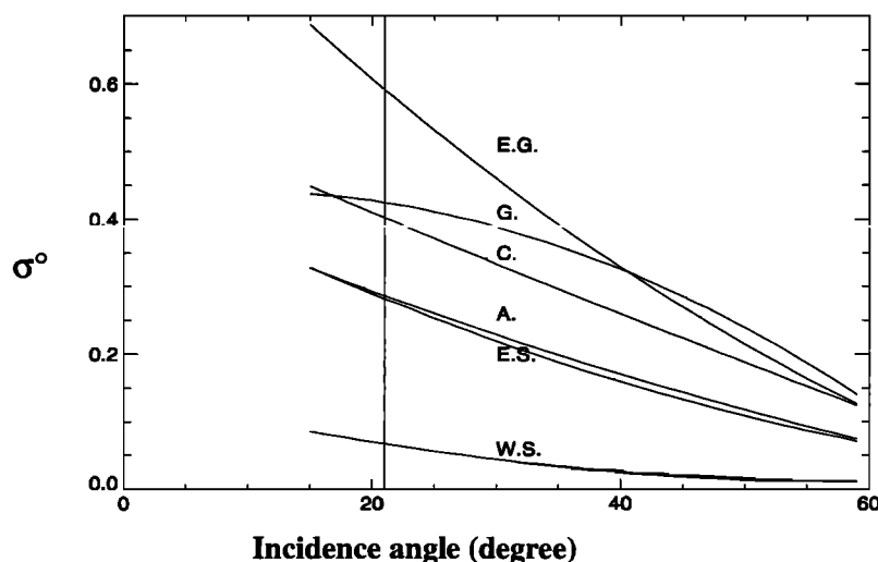
Figure 4. NSCAT backscatter over sea ice as a function of incidence angle for the six selected sectors: EG, east Greenland; G, Greenland; C, central Arctic; A, Alaska; ES, east Siberia; and WS, west Siberia.
