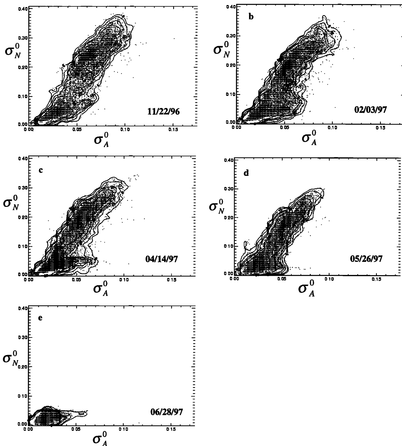
Figure 7. Scatterplots of Ku band versus C band \sigma^0 over the Arctic Ocean sea ice for (a) November 1996 and (b) February, (c) April, (d) May, and (e) June 1997.
