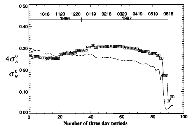
Figure 11. Time series of backscatter values for the central Arctic sector from September 9, 1996, to June 27, 1997. Solid line is Ku band \sigma^0 ; squares denote C band \sigma^0 multiplied by 4.
