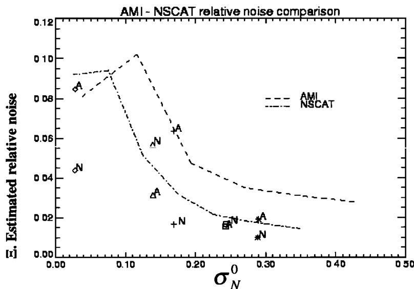
Figure 6. Relative noise of AMI and NSCAT as a function of the Ku band \sigma^0 for central Arctic (squares), west Siberia (diamonds), east Siberia (triangles), Alaska (pluses), and Greenland (stars). Dashed lines correspond to the whole Arctic Ocean sea ice.
