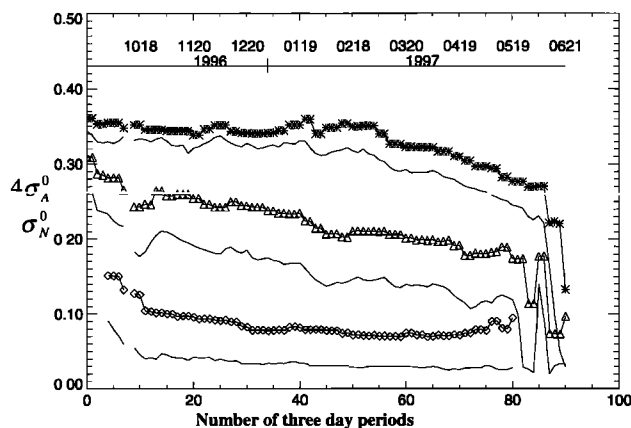
Figure 9. Time series of backscatter values from September 9, 1996, to June 27, 1997. C band \sigma^0 multiplied by 4 is shown for west Siberia (diamonds), east Siberia (triangles), and Greenland (stars); Ku band \sigma^0 is shown by solid lines for the corresponding sectors.
