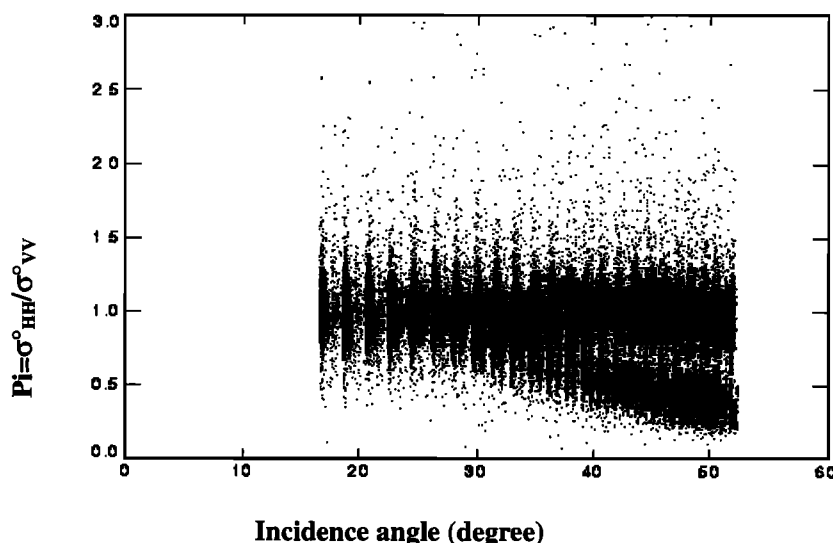
Figure 1. Typical scatterplot of the polarization Index ( P_i ) as a function of incidence angle over the Arctic Ocean.
