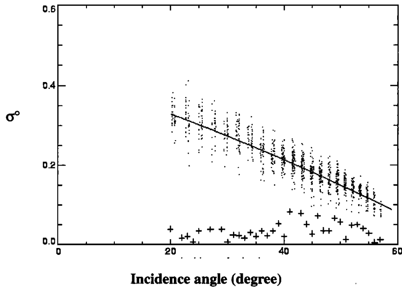
Figure 3. Typical distribution of backscatter data as a function of incidence angle for a single beam and over a selected area. Case presented is from the Alaska sector, beam 2, October 14–16, 1996. The number of data points (pluses) is divided by 1000.
