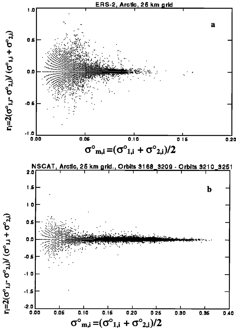
Figure 5. Scatterplot of the relative difference of backscatter r_i as a function of the mean backscatter for the whole Arctic Ocean sea ice for (a) C band and (b) Ku band.
