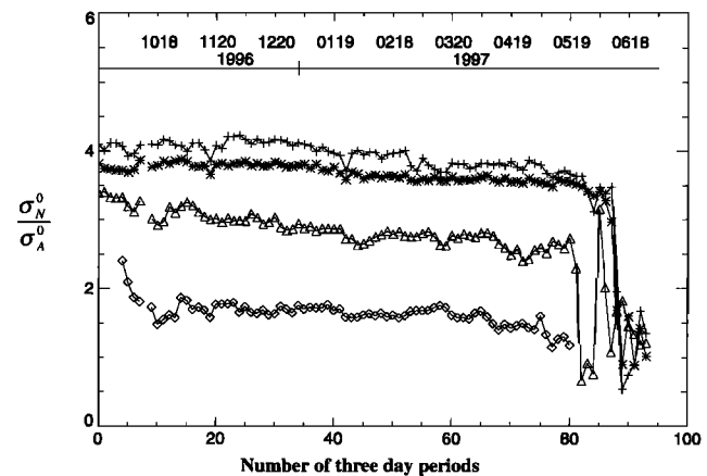
Figure 10. Time series of the ratio of Ku band to C band backscatter values from September 9, 1996, to June 27, 1997, for east Greenland (pluses), Greenland (stars), east Siberia (triangles), and west Siberia (diamonds).
