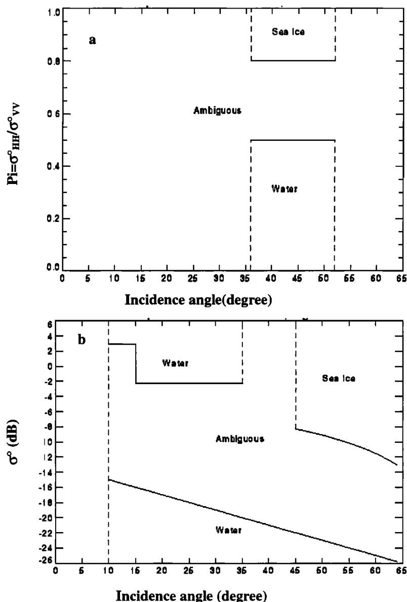
Figure 2. Schematic of the criteria used to discriminate sea ice from open water using NASA scatterometer (NSCAT) data, showing (a) polarization index and (b) backscatter levels as a function of incidence angle.
