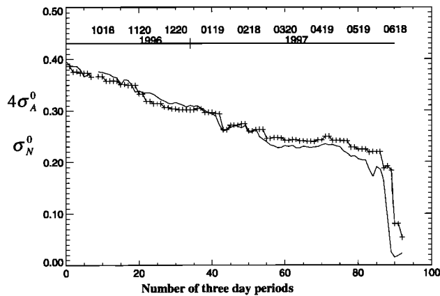
Figure 8. Time series of backscatter values for the east Greenland sector from September 9, 1996, to June 27, 1997. Solid line is Ku band \sigma^0 ; pluses denote C band \sigma^0 multiplied by 4.
