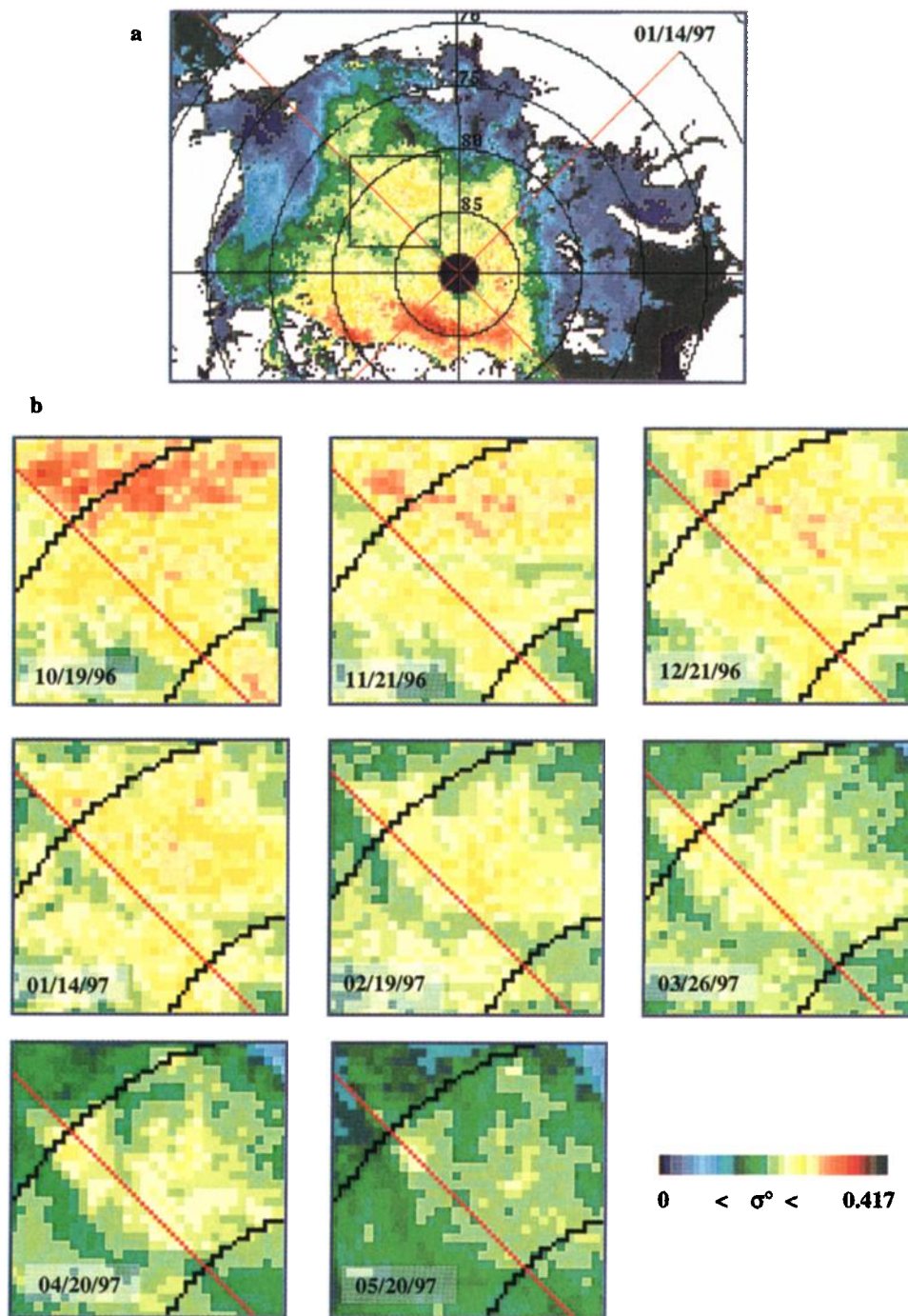
Plate 3. Three-day NSCAT backscatter map at 40° incidence angle centered on January 14, 1997, showing (a) the area studied and (b) time series of the zooms from October 19, 1996, to May 20, 1997.
