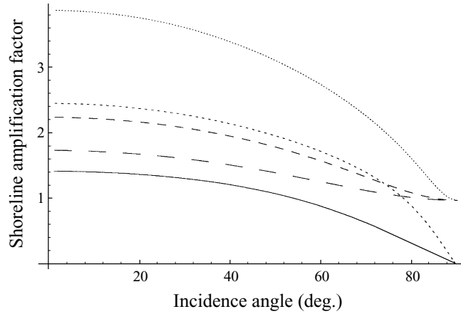
FIGURE 3. Maximum shoreline amplification factor as a function of incidence angle. Full line, beach slope 45^\circ ; broken line, beach slope 30^\circ ; dashed line, beach slope 18^\circ ; dotted line, beach slope 15^\circ ; finely dotted line, beach slope 6^\circ .
