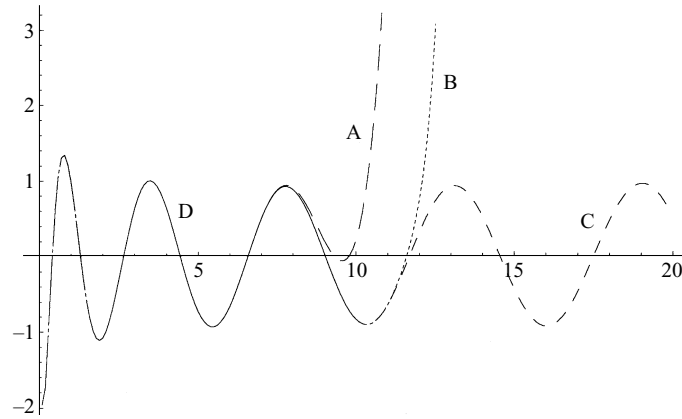
FIGURE 4. Numerical behaviour of near-field expansion of singular wave potential (from equation (8.4)). Case of 6^\circ beach with near-normal ( 1^\circ ) wave incidence: Broken line A, 16 terms of expansion; dotted line B, 32 terms of expansion; dashed line C, 72 terms of expansion; full line D, exact solution from two-dimensional theory shown for R < 10 .
