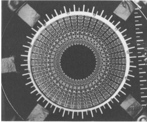
FIGURE 3. The influence of sidewall geometry at low viscosity. A single standing-wave Bessel mode J_{21} appears on the surface of water in a circular container of 12 cm diameter and depth 0.29 cm subjected to sinusoidal vertical vibration at 75 Hz.
