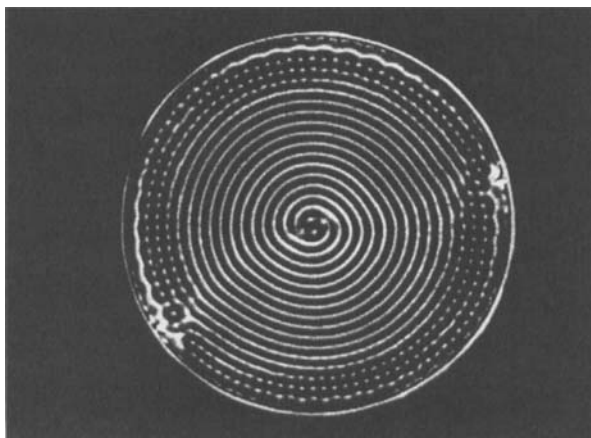
FIGURE 10. Spiral pattern after abrupt transition. Different experimental runs produce circles or spirals, apparently at random. The double spiral includes two defects at the boundary. The pattern rotates counterclockwise with a period of about one minute.
