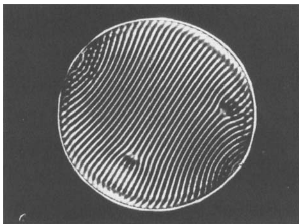
FIGURE 8. Defect-pair generation in a circular container. The fluid and forcing frequency are the same as for figure 6, with slightly higher forcing amplitude. Defect pairs are spontaneously produced near the centre and propagate outward.
