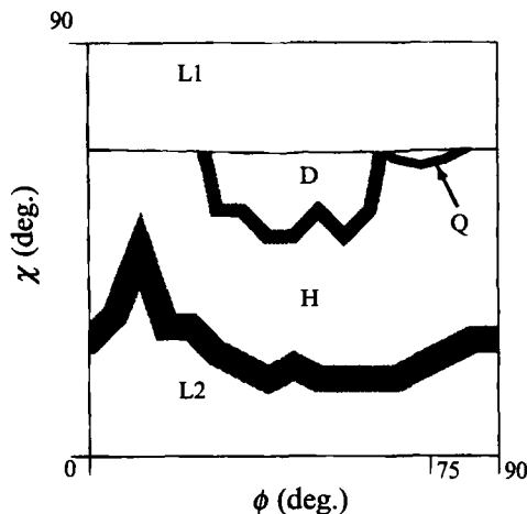
FIGURE 11. Patterns arising near the primary instability. For each point in this plane, i.e. for fixed \phi and \chi of the vertical acceleration f(t) = a[\cos(\chi)\cos(4\omega t) + \sin(\chi)\cos(5\omega t + \phi)] with \omega/2\pi = 14.6 Hz, instability of the flat surface is obtained by slowly increasing the amplitude a . This figure shows which pattern is observed just above the primary transition from the flat surface: L1, lines with k \approx 8.8 \text{ cm}^{-1} ; Q, twelvefold quasi-pattern; H, hexagons; L2, lines with k \approx 7.5 \text{ cm}^{-1} ; D, dynamic states including breaking of the surface. The quasi-pattern is found only very near the bicriticality (the horizontal line) for \phi near 75^\circ . The figure is compiled from observations on a 16 \times 17 grid of (\phi, \chi) values. Thick grey lines indicate regions where two patterns are in competition or are simultaneously present near the primary transition.
