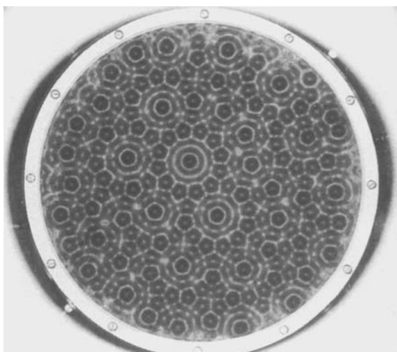
FIGURE 18. Higher-frequency quasi-pattern. The existence of Q does not depend strongly on frequency. Here \omega/2\pi = 28 Hz, \phi = 68.4^\circ and \chi = 72^\circ .
