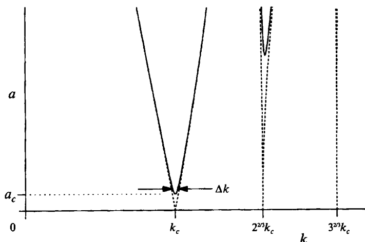
FIGURE 2. Resonance tongues for the Faraday problem with f(t) = a \cos(2\omega t) , from tabulated results for the Mathieu equation, are shown for the infinite-depth capillary dispersion relation \omega_0^2 = (\sigma/\rho)k^3 . Dashed lines are inviscid stability boundaries. Solid lines are stability boundaries for a small viscosity \nu , with damping \delta = 2\nu k^2 . The critical forcing acceleration is a_c for the subharmonic tongue at k_c . The band of unstable wavenumbers \Delta k is shown here for \mu \equiv (a - a_c)/a_c = 0.3 .
