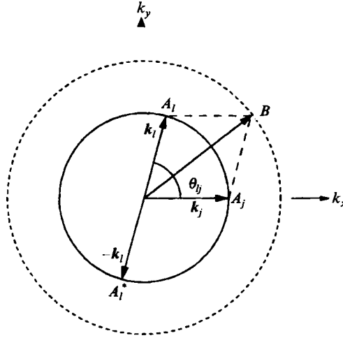
FIGURE 4. Influence of the harmonic resonance on the cubic coefficient \beta(\theta_{ij}) . For low-viscosity capillary waves, the mode B will resonate spatially and temporally with the quadratic interaction of A_j and A_i when \theta_{ij} is such that |k_j + k_i| = 2 \cos(\theta_{ij}/2) k_c = 2^{2/3} k_c , corresponding to the harmonic response tongue of figure 2. The temporal Floquet multiplier is -1 for the subharmonic modes A_j , A_i , and +1 for the harmonic mode B . If B is slightly damped, it can be slaved to the A modes at quadratic order, but at cubic order it will strongly affect \beta(\theta) at the angle \theta = 74.9^\circ .
