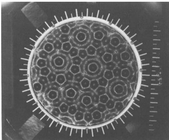
FIGURE 17. Quasi-pattern of twelvefold symmetry. Photograph of the pattern Q, which has long-range order but no spatial periodicity. The long-range order may be seen by viewing the photograph at a glancing angle; in certain directions there are parallel lines which traverse the container. The parameters are as in figures 12 and 16 with \chi = 65^\circ .
