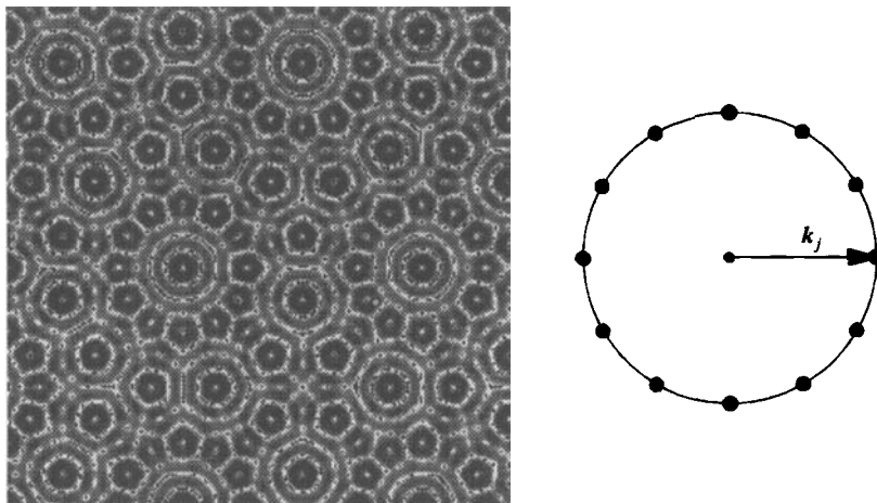
FIGURE 23. Computer-generated quasi-pattern is a linear superposition of twelve wavevectors k_j . The effect of the experimental visualization is approximated by time-averaging the reflected light that would reach the camera from each point on the surface. No fivefold or tenfold symmetry exists, despite the apparent pentagons.
