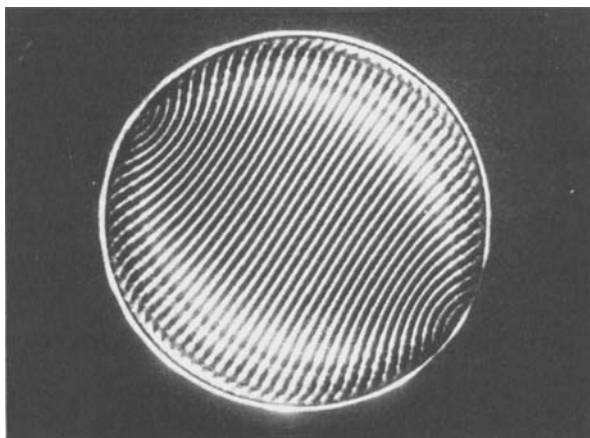
FIGURE 6. Single-frequency forcing at high viscosity. A pattern of essentially parallel lines is observed with a mixture of 88 % glycerol and 12 % water, having \nu \approx 1.00 \text{ cm}^2 \text{ s}^{-1} . The forcing frequency 2\omega/2\pi is 80 Hz.
