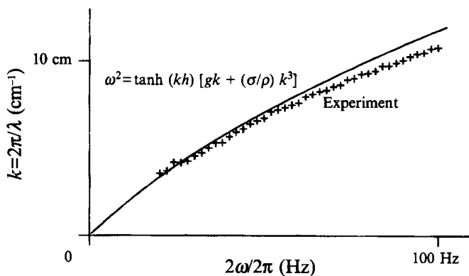
FIGURE 7. Measured dispersion relation (crosses) for lines at viscosity \nu = 1.00 \pm 0.05 \text{ cm}^2 \text{ s}^{-1} is close to the theoretical zero-viscosity result (solid line). The values \sigma = 65 \text{ dyn cm}^{-1} and \rho = 1.22 \text{ g m}^{-3} for the theoretical curve are literature values for the glycerol/water mixture.
