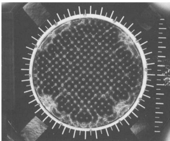
FIGURE 22. Squares observed with the frequency ratio 3/5 . At this viscosity, the individual frequencies each produce lines; mixing the two frequencies results in squares for broad parameter ranges of \chi and \phi .
