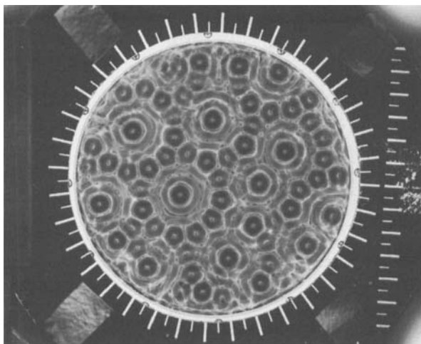
FIGURE 21. Quasi-pattern observed with frequency ratio 6/7 . Similar twelvefold quasi-patterns are observed for frequency ratios 4/7 and 8/9 . They are found by experimentally locating the bicritical mixing angle \chi and then slowly varying the phase \phi , with a fixed just above the stability threshold.
