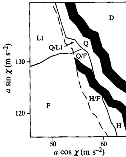
FIGURE 16. Transitions among the flat surface F, quasi-pattern Q, hexagons H and lines L1. With increasing a , the flat surface becomes unstable at one of the solid lines bounding region F. The resulting pattern can be H, Q or L1, depending on \chi . Hysteresis is shown by the dashed line; in region H/F both H and F are stable, and similarly for Q/F. The solid line separating L1 and Q shows the transition L1 to Q, with hysteresis shown by the dashed line; in region Q/L1 both Q and L1 are stable. The grey band separating H and Q is a region of competition in which the two patterns coexist and/or oscillate slowly. Region D indicates a dynamic and/or disordered state; the transition from an ordered quasi-pattern to D (the grey band separating Q and D) involves slow, irregular dynamics in which the quasi-pattern spontaneously breaks up and reforms.
