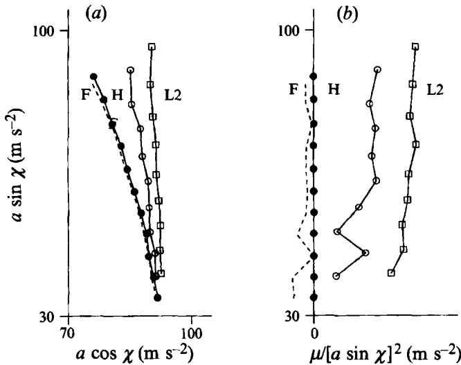
FIGURE 14. Hexagons-to-lines transition. In (a), the phase diagram is plotted in the plane of the two forcing amplitudes, and in (b) the same data are shown but with the horizontal axis \mu/[a \sin \chi]^2 , where \mu \equiv (a - a_c)/a_c . Solid circles show the transition from the flat surface F to hexagons H as \mu is slowly increased. Dashed lines show the transition from H to F for decreasing \mu . Open circles and squares delimit the region in which the hexagon-to-lines transition takes place; squares show the final disappearance of hexagons as \mu is increased, while circles show the final disappearance of lines as \mu is decreased. The width of the region of stable hexagons is approximately proportional to the square of the amplitude a \sin \chi , as shown by the nearly vertical transition boundary in (b), especially in the upper portion of the diagram where the width is much larger than parameter fluctuations due to temperature.
