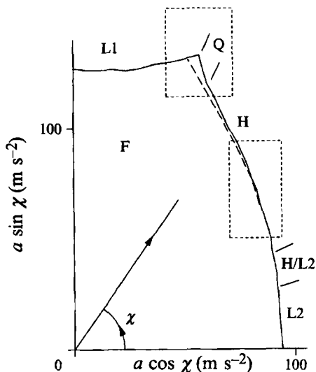
FIGURE 12. Stability boundaries for \phi = 75^\circ in the (a, \chi) -plane, showing the primary transition from the flat surface (solid line), hysteresis (dashed line), and the pattern which develops just above a = a_c(\chi) . The instability is produced by fixing \chi and increasing a as shown by the arrow. Dashed boxes correspond to figures 14 and 16.
