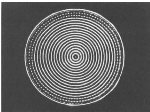
FIGURE 9. Circular pattern after abrupt transition. The flat surface becomes unstable after a rapid increase in the forcing acceleration a , giving rise to circular waves. The pattern is a result of the circular sidewall. Once created, it persists indefinitely.
