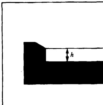
FIGURE 5. Sidewall boundary condition. The aluminium sidewall has a corner where the slope changes discontinuously from 90^\circ to 30^\circ . With a glycerol/water mixture the contact line becomes pinned at the corner, making possible the preparation of a flat surface with no meniscus. The 30^\circ 'beach' makes the fluid fall back into place if the contact line is temporarily disrupted.
