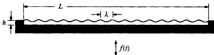
FIGURE 1. Basic hydrodynamic problem. A rigid container of depth h and horizontal dimension L (in both horizontal directions) is filled with an incompressible Newtonian fluid of density \rho and kinematic viscosity \nu . The surface tension on the free upper surface is \sigma . The container is subjected to oscillatory vertical acceleration f(t) . Standing waves of wavelength \lambda appear on the surface when the amplitude a of the forcing exceeds a threshold value a_c .
