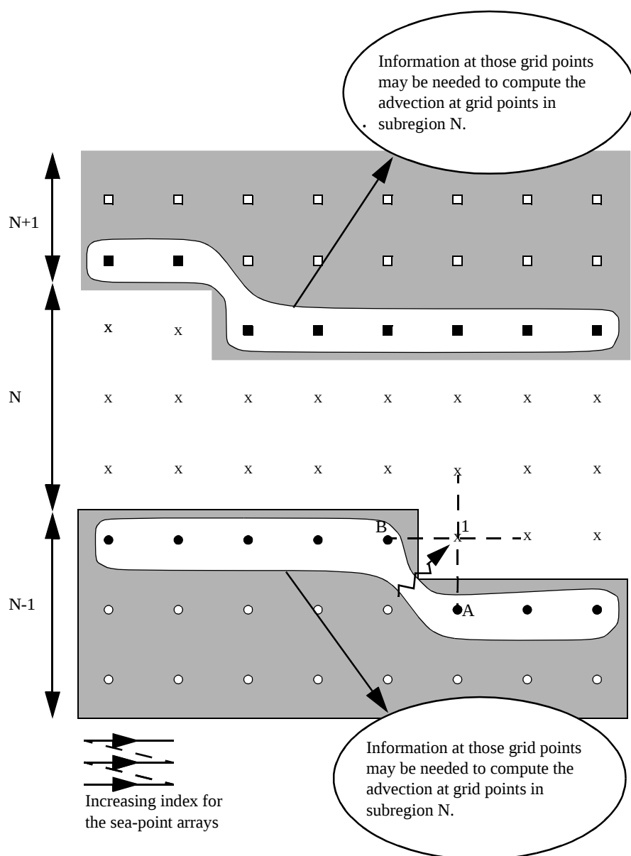
Figure 6.2 Domain decomposition.
