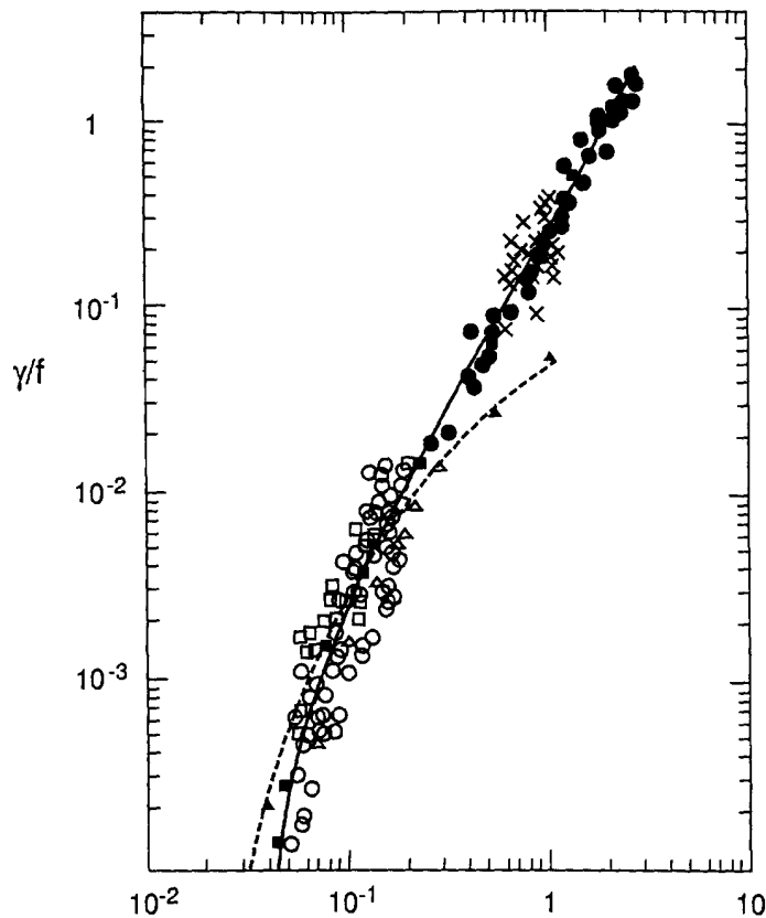
Figure 3.1 Comparison of theoretical growth rates with observations by Plant (1982) (full line): Miles' theory; (full dots): parametrization of Miles' theory (3.3); dashed line: the fit by Snyder et al. (1981) .
