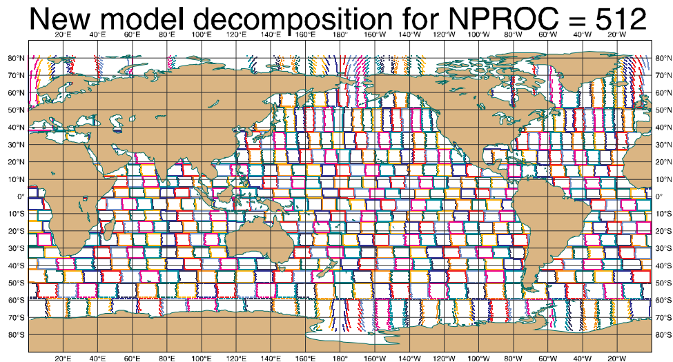
Figure 6.6 2-D decomposition of the WAM model 0.5° irregular lat-long grid for 512 processors. The different colour symbols indicate grid points sharing information with neighbouring PE's.
