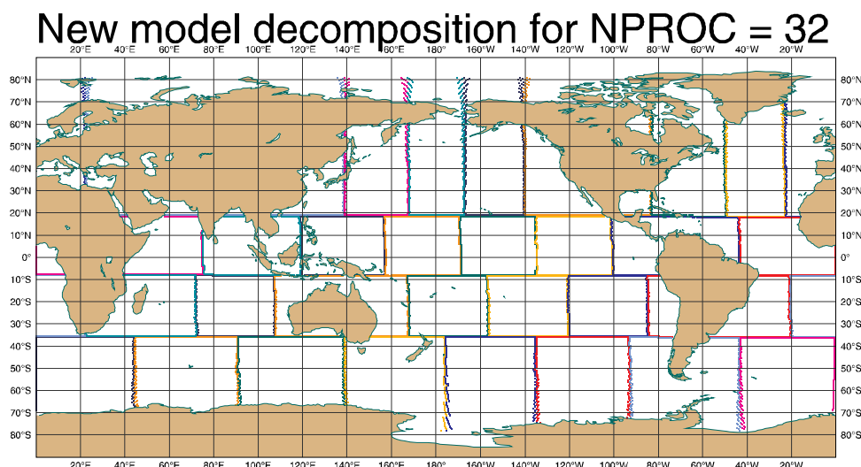
Figure 6.5 2-D decomposition of the WAM model 0.5° irregular lat-long grid for 32 processors. The different colour symbols indicate grid points sharing information with neighbouring PE's.
