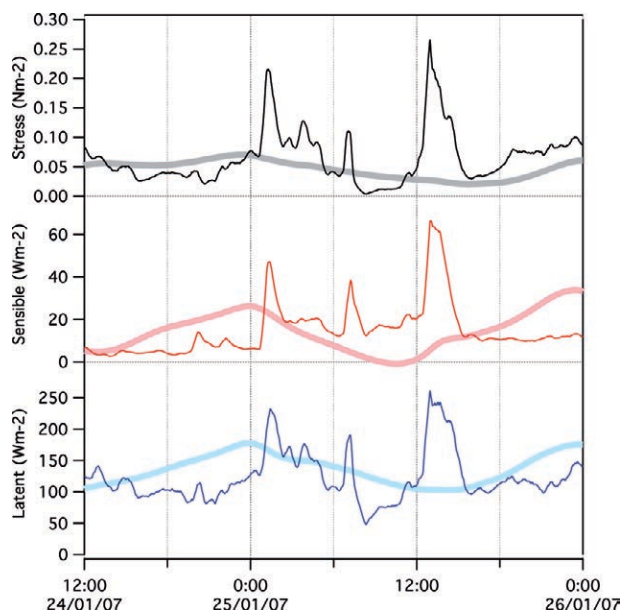
FIG. 4. Surface fluxes computed with the COARE 3.0 bulk algorithm for the time series shown in Fig. 3 with thick lines for ECMWF variables. (from top to bottom) Wind stress (black), turbulent sensible heat flux (red), and turbulent latent heat flux (blue).
