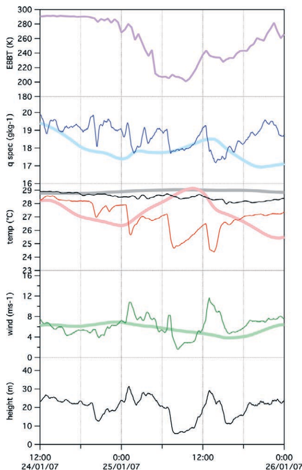
FIG. 3. Time series of Aeroclippers 4 measurements and of Meteosat IR brightness temperature for the red trajectory reported in Fig. 2. (from top to bottom) IR brightness temperature at the top of the atmosphere (purple), 10-m specific humidity (blue), 40-cm ocean temperature (black) and 10-m air temperature (red), 10-m wind (green) deduced from the Aeroclippers displacement and relative wind measurements, and height of the Aeroclippers atmospheric measurements (black). These curves are 30-min running means of the original 1-min time step. 30 min correspond to a displacement of the Aeroclippers of 3.6 km (8.1 km) for a 10-m wind of 5 m s -1 (10 m s -1 ). The thick lines represent the ECMWF atmospheric variables at 10 m and the SST used in the model along the path of the Aeroclippers.
