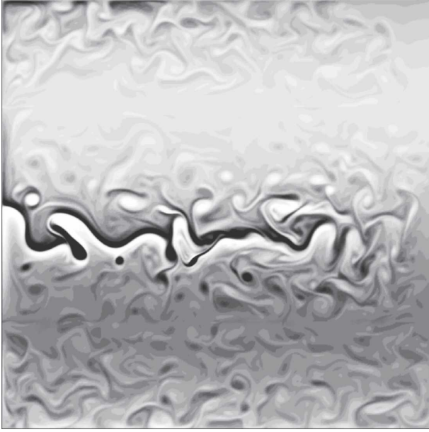
FIG. 4. Wind stress curl [\mathbf{k} \cdot (\nabla \times \boldsymbol{\tau}_1)] for the snapshot corresponding to Fig. 1b. Lighter shades correspond to cyclonic forcing.
