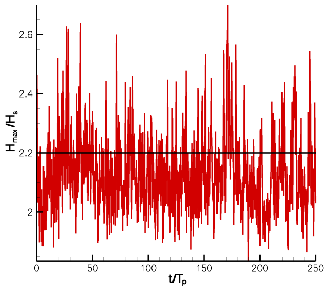
Fig. 11. Evolution of H_{\max} / H_s during time of simulation, directionality n=2 .
