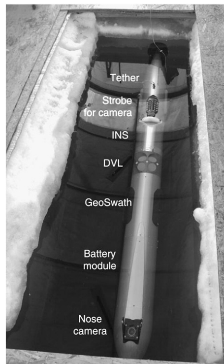
Fig. 2. The Gavia AUV, ballasted for upward-looking operation, in the deployment ice hole. Various module functions are indicated. The vehicle is 2.9 m long in this configuration and 20 cm in diameter.
