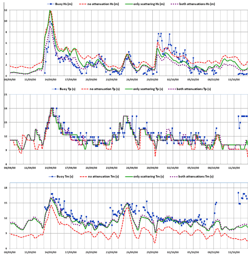
Fig. 4. Significant wave height (top panel), peak period (middle panel) and mean period (bottom panel) over the period of breakup. Results are shown for the buoy observations (blue squares), and the WAM results at the buoy location, for the un-attenuated WAM model (red dashed line), the scattering-only attenuation scheme (green solid line) the combine scattering + drag scheme (magenta dotted line). (For interpretation of the references to color in this figure legend, the reader is referred to the web version of this article.)
