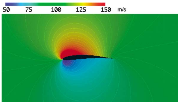
Fig. 7. Flow speed v_0 .
