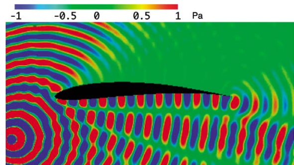
Fig. 8. f = 2 kHz, Acoustic pressure field p_1 .
