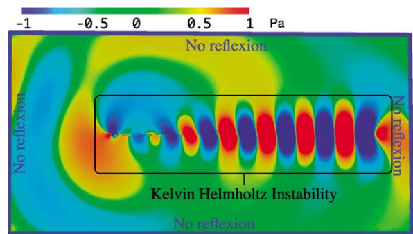
Fig. 6. Kelvin-Helmholtz instability, p_1 .
