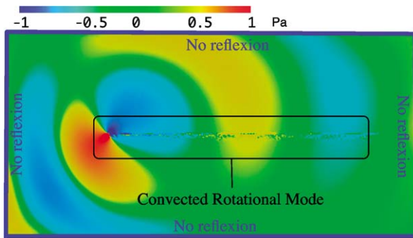
Fig. 5. Acoustic and Rotational Modes, p_1 .
