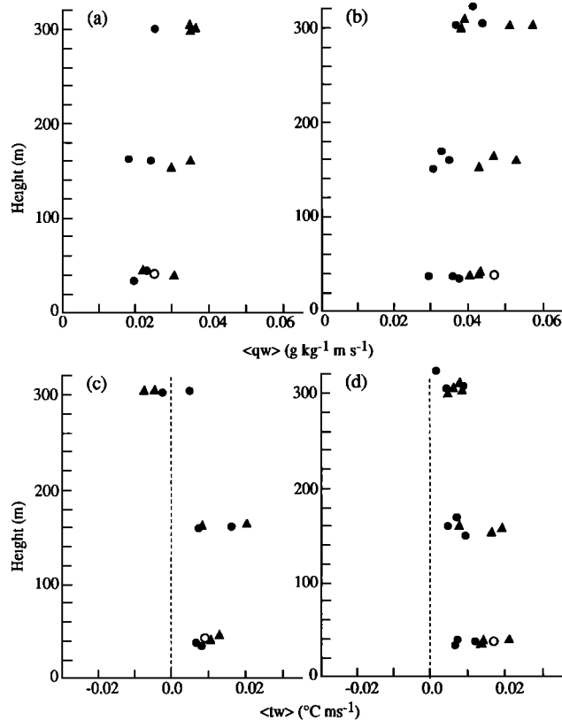
Figure 7. (a,b) Humidity flux \langle q_w \rangle and (c,d) temperature flux \langle t_w \rangle at three heights in the boundary layer, measured by the BMO aircraft during flights (a and c) H760 and (b and d) H762. (See Table 2 for values at 30 to 40-m height.) Solid circles indicate data collected on leg CD, triangles on leg GH, and open circles on leg AB.
