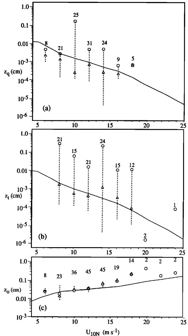
Figure 11. Log of (a) water vapor roughness length z_q , (b) temperature roughness length z_t , and (c) roughness length z_0 for the UW data and as predicted by Liu et al. [1979] using the model of Brown and Liu [1982] (solid lines). Data have been combined in 2 m/s wind speed categories. Within each category, triangles represent the median value, dotted lines the interquartile range, and circles the mean; the number of points in each category is shown.
