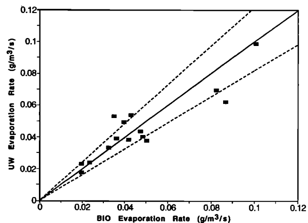
Figure 5. Comparison of water vapor fluxes measured independently by UW and BIO sensors during same time intervals. Most of the points lie within dashed lines Y = 1.24X , X/1.24 , indicating estimated experimental error.
