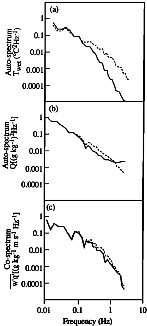
Figure 2. (a) Spectra of wet-bulb temperature ( T_{\text{wet}} ), measured (solid line) and simulated (dashed line); see text. (b) Spectrum of water vapor density using the wet-bulb signal adjusted with a time constant of 0.756 s (solid line) and the Lyman \alpha humidimeter (dashed line). (c) Cospectrum of vertical velocity and water vapor density for the corrected psychrometer (solid line) and the Lyman \alpha (dashed line).
