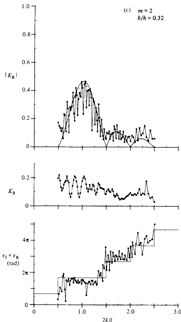
FIGURE 6. Results for the reflection coefficients both of the ripple patch ( |K_R| ) and of the beach ( K_B ) for: (a) m = 10 ripples ( b/h = 0.16 ); (b) m = 4 ripples ( b/h = 0.32 ); (c) m = 2 ripples ( b/h = 0.32 ). The solid and broken curves represent the predictions of the uncorrected and corrected theory respectively. Estimates of the sum of the phase angles \epsilon_I + \epsilon_R are shown for the case of m = 2 ripples.
