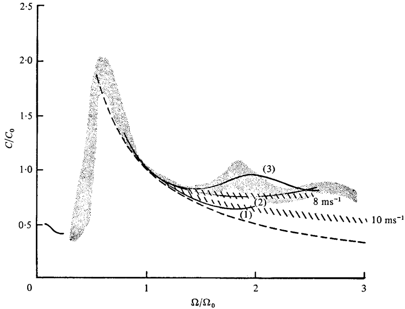
FIGURE 13. Comparisons of calculations with ocean and laboratory data collected by Ramamonjariosa & Giovanangeli (1978). \square , laboratory data (Ramamonjariosa & Coantic 1976); \boxtimes , ocean data (Ramamonjariosa & Giovanangeli 1978). —, nonlinear theory: (1), Yefimov spectrum, k_0 a_0 = 0.03 ; (2), Yefimov spectrum, k_0 a_0 = 0.07 ; (3), Bretschneider, \sigma = 0.07 , k_0 a_0 = 0.1 . ---, linear theory.
