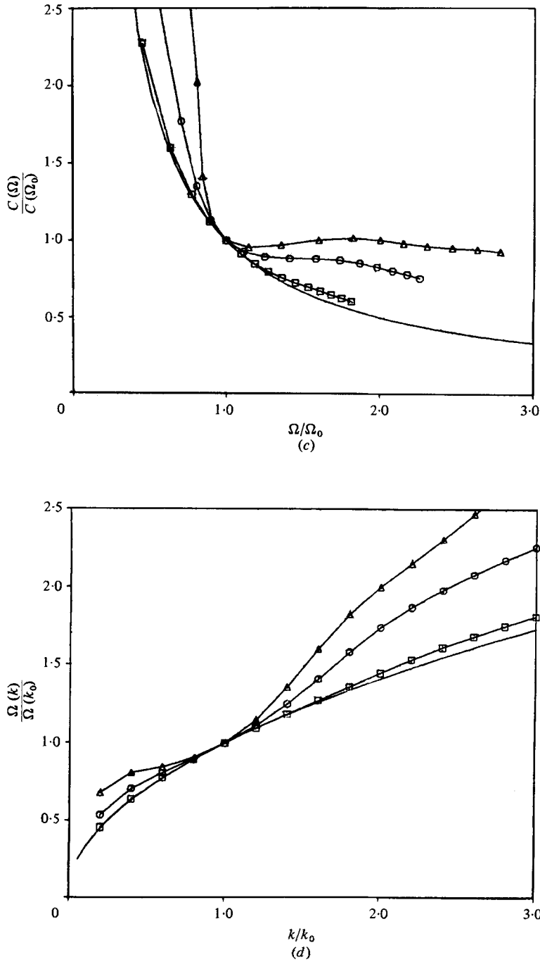
FIGURE 4. Component-phase-speed and dispersion-relation calculations for continuous spectra (Lorentzian form) with fixed bandwidth, \sigma = 0.20 and varying nonlinearity. (a) Dimensionless wavenumber spectra. (b) Normalized component phase speed as a function of wavenumber. (c) Normalized component phase speed as a function of frequency. (d) Normalized dispersion relation. \square , ka = 0.01 ; \circ , ka = 0.10 ; \triangle , ka = 0.20 . —, linear case.
