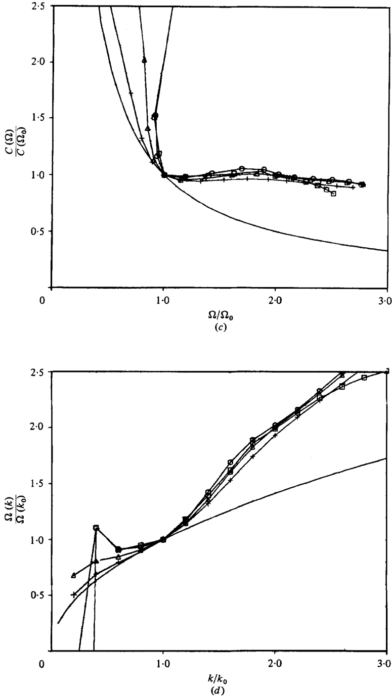
FIGURE 6. Component-phase-speed and dispersion-relation calculations for continuous spectra (Lorentzian form) with fixed nonlinearity (ka)_{rms} = 0.20 and varying bandwidth. (a) Dimensionless wavenumber spectra. (b) Normalized component phase speed as a function of wavenumber. (c) Normalized component phase speed as a function of frequency. (d) Normalized dispersion relation. \square , \sigma = 0.05 ; \circ , \sigma = 0.10 ; \triangle , \sigma = 0.20 ; + , \sigma = 0.30 . —, linear case.
