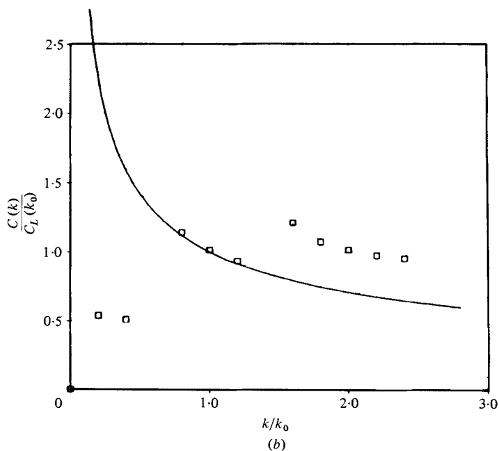
FIGURE 1. Phas-speed calculations for a modulated wavetrain with (ka)_{\text{rms}} = 0.10 . (a) Dimensionless spectrum F(k)/F(k_0) versus dimensionless wavenumber k/k_0 . (b) Component phase speed normalized by linear phase speed k_0 , C(k)/C_L(k_0) , versus dimensionless wavenumber k/k_0 . —, linear case.
