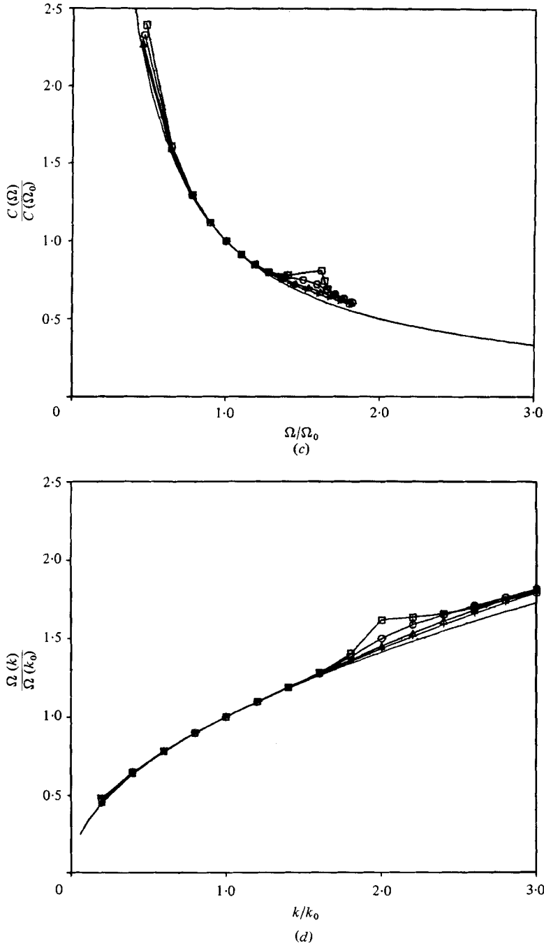
FIGURE 5. Component-phase-speed and dispersion-relation calculations for continuous spectra (Lorentzian form) with fixed nonlinearity (ka)_{\text{rms}} = 0.01 and varying bandwidth. (a) Dimensionless wavenumber spectra. (b) Normalized component phase speed as a function of wave-number. (c) Normalized component phase speed as a function of frequency. (d) Normalized dispersion relation. \square , \sigma = 0.05 ; \circ , \sigma = 0.10 ; \triangle , \sigma = 0.20 ; + , \sigma = 0.30 . —, linear case.
