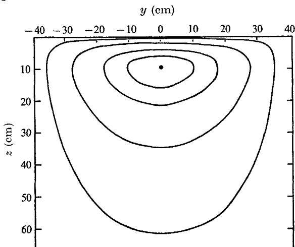
FIGURE 4. The streamlines f(z) \cos 2ly = \text{constant} , for the symmetric interaction m = 0.1 \text{ cm}^{-1} , l = 0.02 \text{ cm}^{-1} , \alpha = 100 \text{ cm} .
