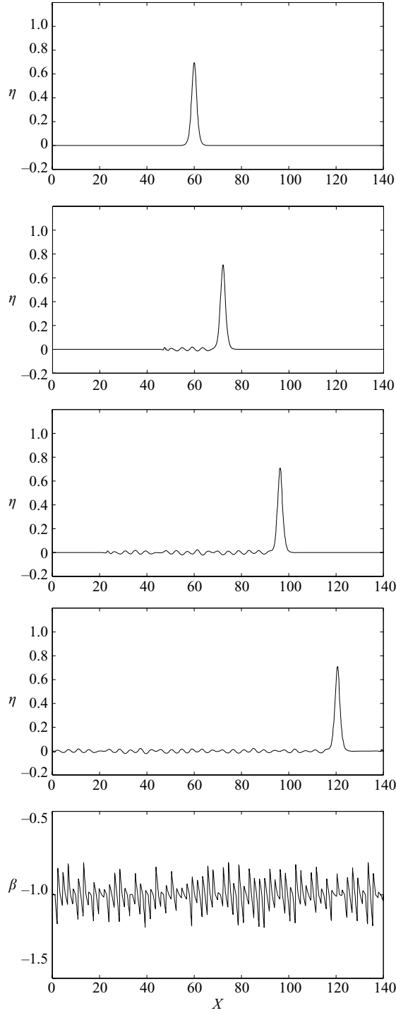
FIGURE 5. Profiles of the free surface \eta for \varepsilon = 0.2 ( h = 1 ) at t = 0, 12, 36, 60 showing the development of a scattered component. The vertical scale has been enlarged by a factor \varepsilon^{-2} . The lower panel represents the corresponding bottom geometry.
