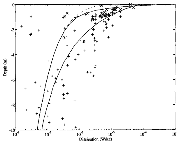
FIG. 8. Comparison of modeled dissipation profiles, for z_0 = 0.1 and 1.0 m, with data from Osborn et al. (1992). Data are from their figures 9b (+) and 9d (x). The dotted line represents the solution for a pure shear generation-dissipation balance.
