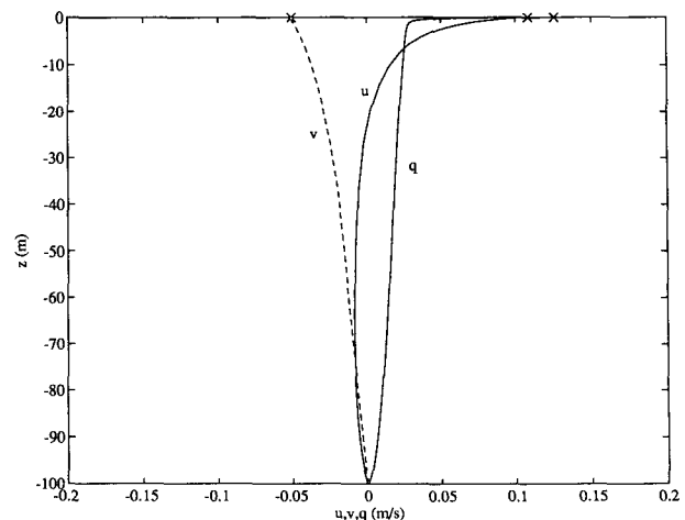
FIG. 4. Profiles of q , u , and v for the full model, with a surface flux of turbulent kinetic energy, shear generation, and dissipation.
