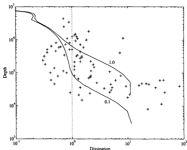
FIG. 7. Comparison of modeled dissipation profiles for z_0 = 0.1 and 1.0 m with data from Agrawal et al. (1992). Dissipation is non-dimensionalized as \epsilon \kappa z / u_*^3 , and depth as z g / u_*^2 . The dotted line represents the conventional law-of-the-wall solution.
