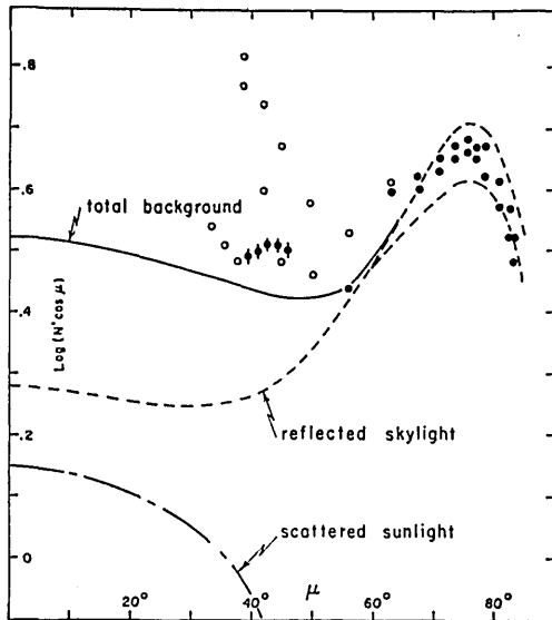
FIG. 6. The background radiation (in arbitrary units) on a moderately rough day (4 Sept 6, \sigma=0.13 ). The solid circles correspond to measurements outside the glitter pattern. The open circles contain some glitter radiation, and lie, therefore, above the background curve. Circles with the vertical line correspond to measurements on the vertical photograph, the other circles to measurements on tilted photograph.
