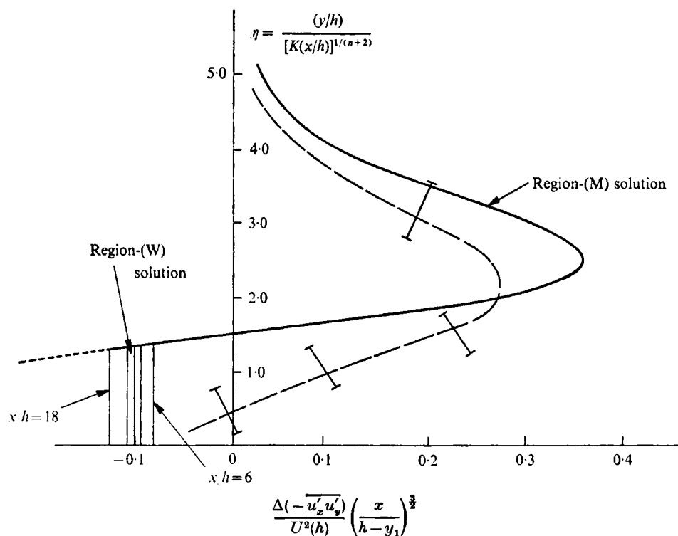
FIGURE 4. Self-preserving profiles of the perturbation Reynolds stress behind a two-dimensional obstacle. — \pm —, experimental curve with scatter bar ( n = 0.125 , h/\delta = \frac{1}{8} ); —, theoretical curve deduced from the theoretical velocity profile.
