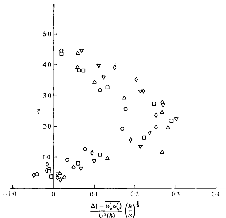
FIGURE 9. Measurements of the perturbation Reynolds stress plotted as a self-preserving profile for the wake behind a two-dimensional block ( n = 0.125 , K = 0.05 , h/\delta \simeq \frac{1}{8} ). x/(h-y_1) : \circ , 7.5; \square , 10.5; \triangle , 13.0; \nabla , 16.1; \diamond , 21.1.
