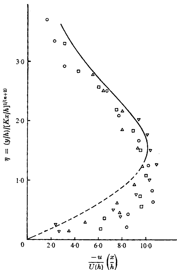
FIGURE 10. Self-preserving plot of Plate & Lin's (1965) velocity measurements behind a 25 \times 100 mm wedge in a turbulent boundary layer on a smooth wall ( n = 0.2 , K = 0.062 , h/\delta \approx \frac{1}{10} ) and the theoretical profile (matching at maximum). x/h : \circ , 24; \square , 32; \triangle , 46; \nabla , 72. —, region-(M) solution; ----, extrapolation of (M) solution into region (W).
