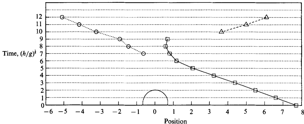
FIGURE 5. As figure 4. Position of crests in time. The incident crest (—) amplitude vanishes at t = 9 . Transmitted wave (·····) has amplitude 0.223 at t = 12 ; reflected wave (-----) has amplitude 0.04 at t = 12 .
