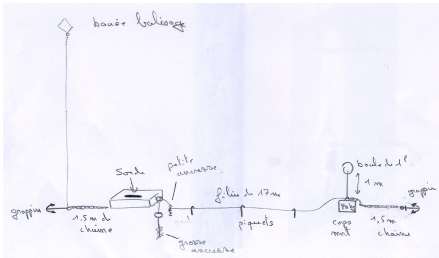
Figure 4.12: Schema of the pressure sensor assembly located around Groix.
