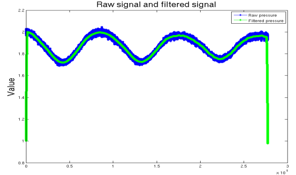
(b) Results of the Hanning filtering. Raw pressure (in blue) and filtered pressure (in green).
